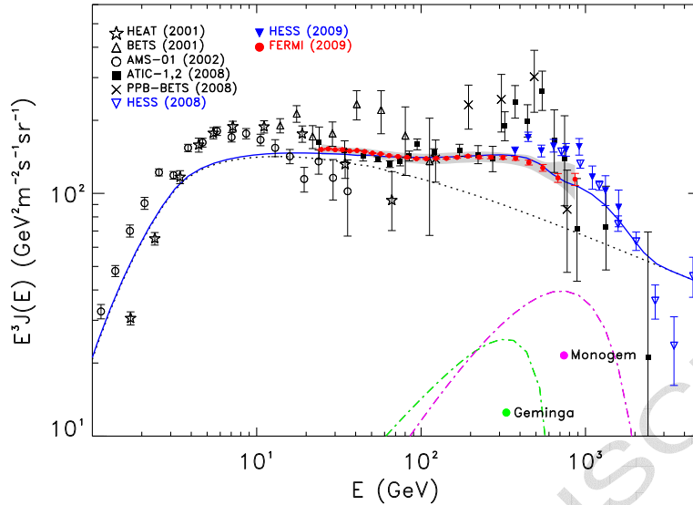
Figure 4: In this figure we represent the electron-plus-positron spectrum (blue continuous line) computed in a case in which only observed pulsars from the ATNF catalogue (Manchester 2005 [46]) with distance d < 1 kpc plus the large-scale Galactic component (GCRE) give a significant contribution. The dominant contribution of Monogem and Geminga pulsars, analytically computed for a representative choice of the relevant parameters (see text) is shown as colored dot-dashed lines, while the GCRE, computed with GALPROP is shown as a black-dotted line. The gray band represents systematic errors on the CRE Fermi-LAT data. Solar modulation is accounted as done in Fig.1.
