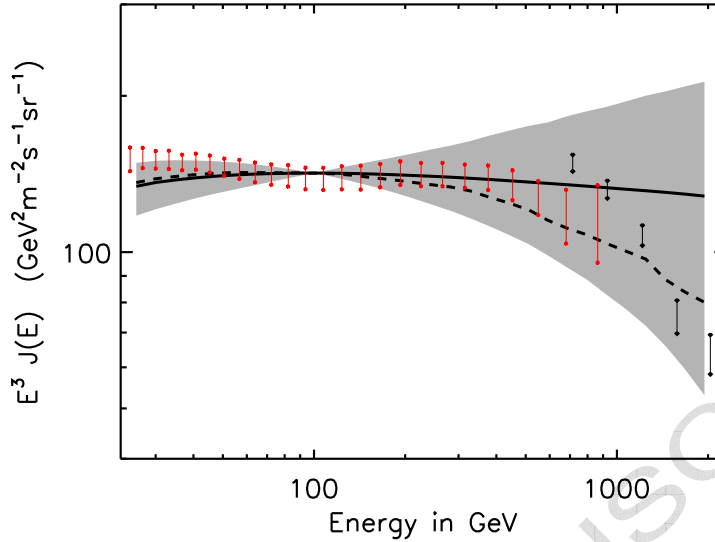
Figure 2: Results of an analytical calculation for stochastic sources, including Gould’s Belt (see Pohl et al. 2003 [33]). The propagation parameters are those of model 1 in Tab. 1, and all spectra are normalized to the fiducial flux at 100 GeV. The solid line gives the average spectrum that one would obtain, if the sources were continuously distributed. The shaded area indicates the 1\text{-}\sigma fluctuation range of the electron flux at each energy. The dashed line indicates one randomly chosen, actual electron spectrum. Fermi-LAT and H.E.S.S. data points are represented in red and black respectively.
