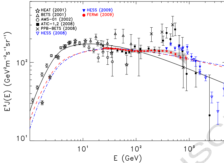
Figure 1: In this figure we compare Fermi-LAT CRE data (Abdo et al. 2009 [27]), as well as several other experimental data sets (HEAT: Du Vernois et al. 2001 [32]; AMS-01: Aguilar et al. 2002 [2]; ATIC: Chang et al. 2008 [7]; PPB-BETS: Tori et al. 2008 [9]; H.E.S.S. 2008: Aharonian et al. 2008, [10]; H.E.S.S. 2009 Aharonian et al. 2009, [11]) with the electron plus positron spectrum modeled with GALPROP under the conditions discussed in Sec.2.1. The gray band represents systematic errors on the CRE spectrum measured by Fermi-LAT. The black continuous line corresponds to the conventional model used in (Strong et al. 2004 [30]) to fit pre-Fermi data model (model 0 in Tab. 1). The red dashed (model 1 in Tab. 1) and blue dot-dashed lines (model 2 in Tab. 1) are obtained with modified injection indexes in order to fit Fermi-LAT CRE data. Both models account for solar modulation using the force field approximation assuming a potential \Phi = 0.55 GV.
