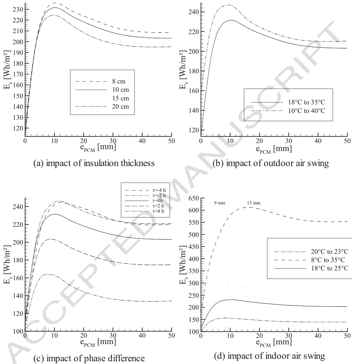
Fig. 7. Impact of various parameters on optimal PCM thickness.
