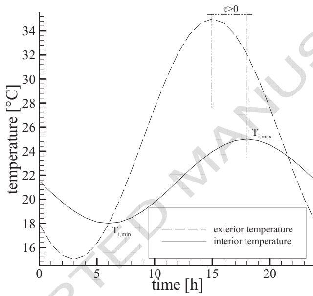
Fig. 5. Air temperature boundary conditions.
