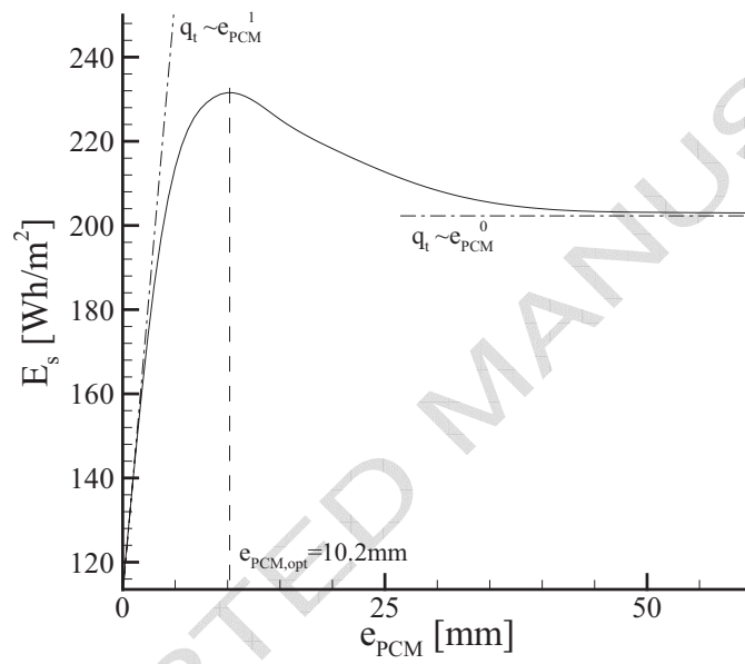
Fig. 6. Results concerning the stored energy in a complete day E_s function of PCM thickness e_{PCM} .
