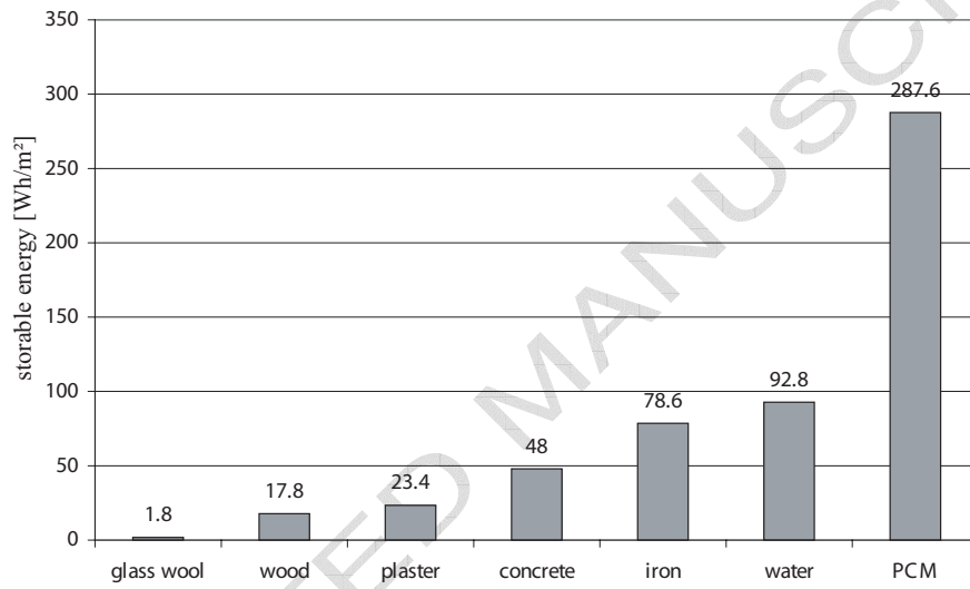
Fig. 8. Maximum storable energy between 18^{\circ}\text{C} and 26^{\circ}\text{C} for 10\text{mm} of material and for 24\text{h} .
