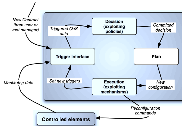
Figure 5 ASSIST framework.
