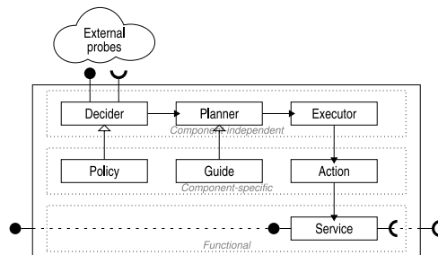
Figure 2 Overall architecture of a Dynaco component.
