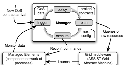
Figure 7: ASSIST framework.
