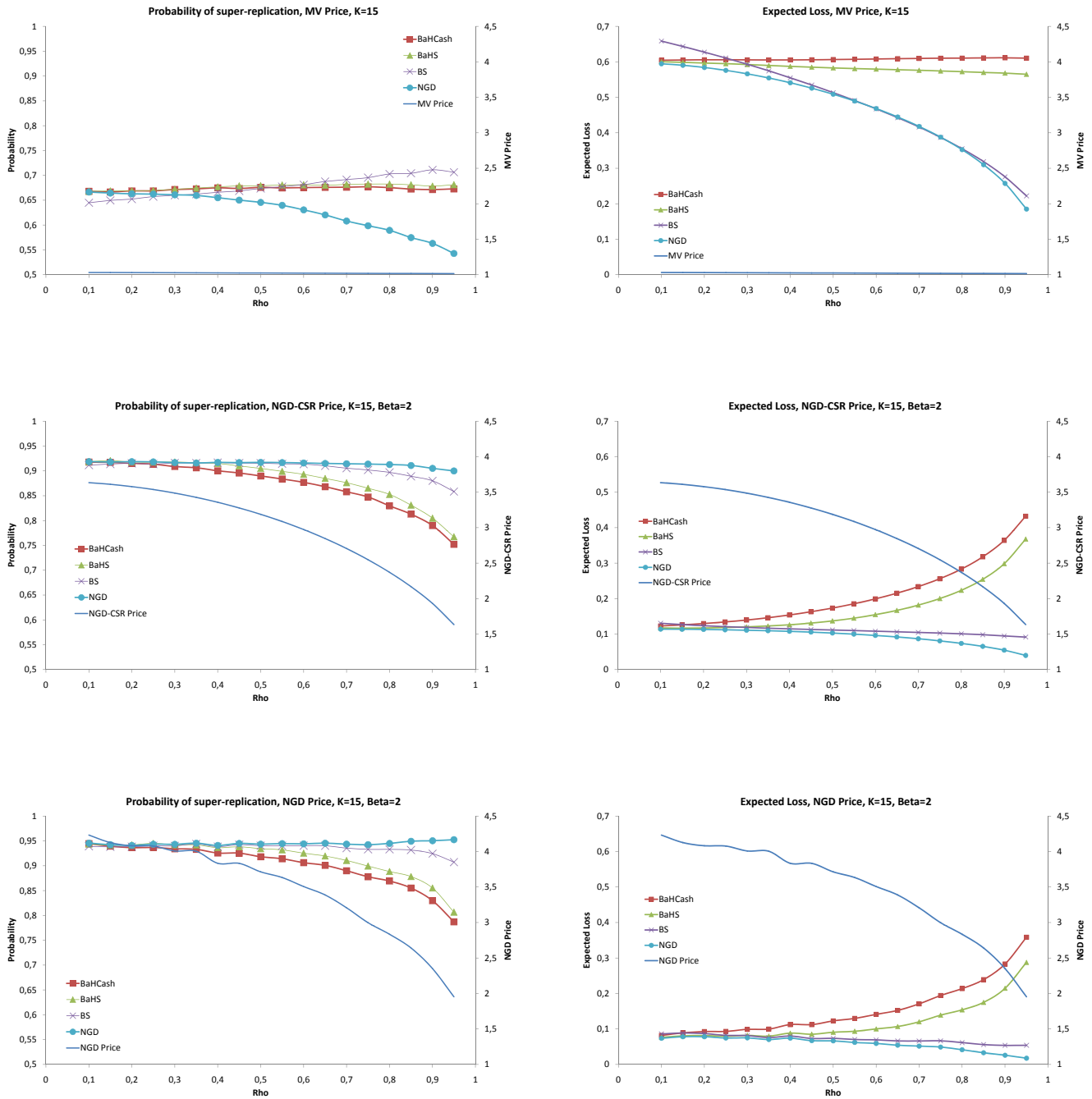
Figure 3: Comparison of the probability of super-replication and expected loss for the different strategies starting from “MV-Price”, “NGD-CSR” and the middle of “NGD-LB” and “NGD-UB”.
