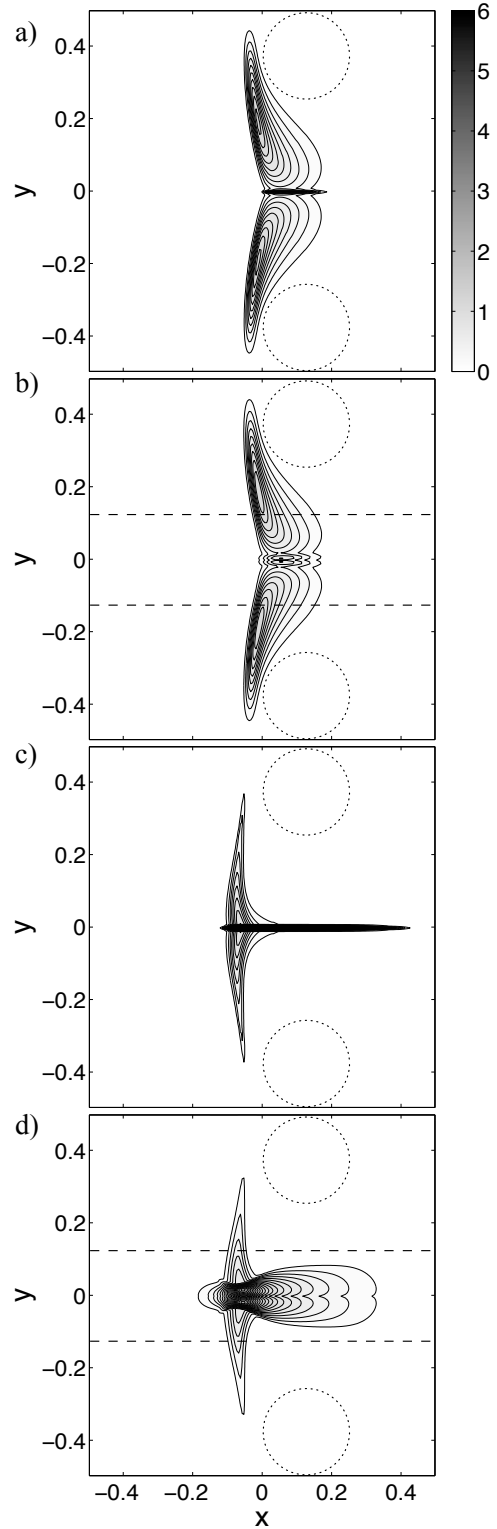
Figure 6: Snapshots of the density for Stokes number St = 13St_c ( 1^{rst} order relaxation scheme, 200 nodes, CFL = 1): pressureless scheme (a, c) and hybrid scheme (b, d). Time t = 0.75 (a, b) and t = 1.1 (c, d). Dotted circles and dashed lines are the limits of the cardinal sinus function of the initial density distribution and the energy source term (b, d) respectively. The maximum density for (c) is 26.81.
