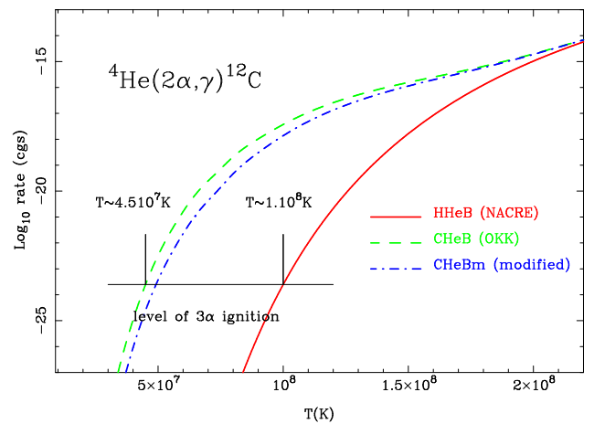
Fig. 1. (Colour online) The NACRE (full) and enhanced Ogata et al. (2009) (dash) triple-alpha reaction rates variations with temperature. With OKK, the temperature of the ignition is about halved. For CHeBm (dot-dash) the correction \log_{10}(\Delta 3\alpha) is arbitrarily reduced by 7% – see Sect. 5.
