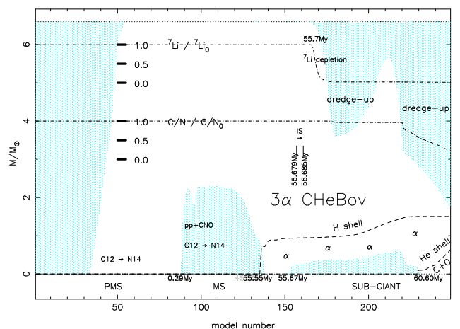
Fig. 8. (Colour online) Evolution of the internal structure of a 6.6M_{\odot} model computed with CHEBov (overshooting).
