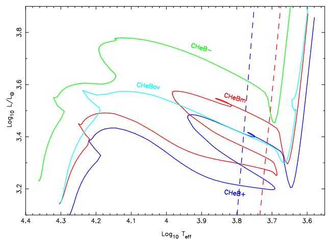
Fig. 7. (Colour online) Comparisons of evolutionary tracks of 6.6M_{\odot} models of numerical experiences, see Sect.5.
