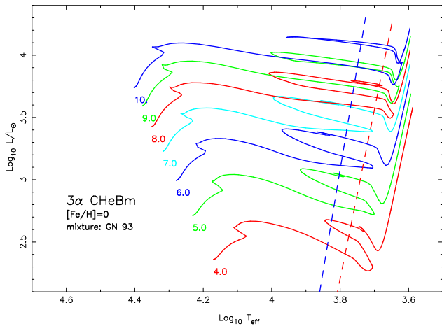
Fig. 5. (Colour online) Same as Fig. 2 left panel for CHEBm (modified 3\alpha OKK rate).
