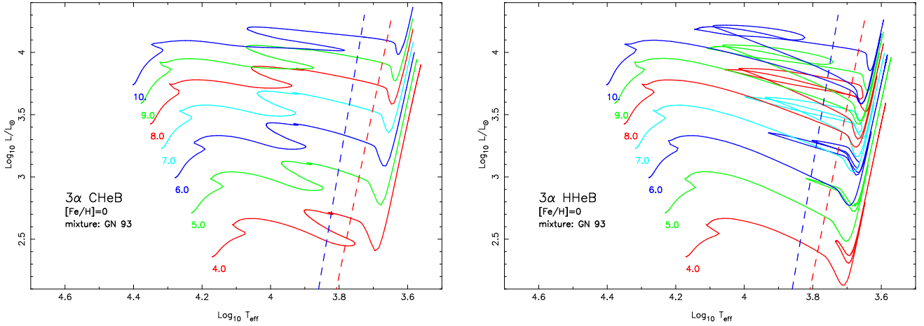
Fig. 2. (Colour online) Left panel: evolutionary tracks computed with cold helium burning (CHeB). Right panel: evolutionary tracks computed with hot helium burning (HHeB). The left and right dashed lines respectively delimit the blue and red sides of the Cepheids instability strip. For clarity only the part of the evolutionary tracks beyond the ZAMS is displayed.
