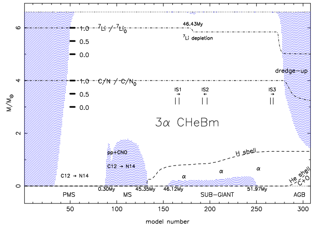
Fig. 6. (Colour online) Evolution of the internal structure of a 6.6M_{\odot} model computed with CHEBm.
