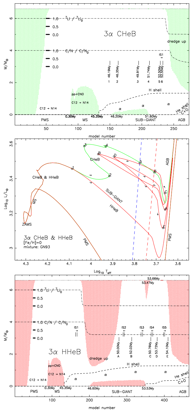
Fig. 3. (Colour online) Evolutions of the internal structure of two models of 6.6M_{\odot} calculated with CHeB (upper panel) and HHeB (lower panel) respectively. The middle panel shows their evolutionary tracks. The models are initialized at PMS (ages in Myr). The blue and red borders of the instability strip are indicated by dashed lines. The crossings of the instability strip are mentioned by IS1, IS2, etc.. Dash-dot lines are the profiles of atmospheric lithium and C/N ratio normalized to their initial values. Convection zones are indicated by filled areas. Other labels are self-explanatory.
