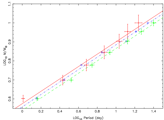
Fig. 4. (Colour online) Mass-period relationship for theoretical models computed with CHeB (dashed), HHeB (full), and CHeBm (dot-dash) respectively.
