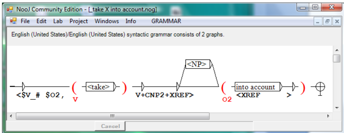
Figure 3: Grammar for take NP into account
