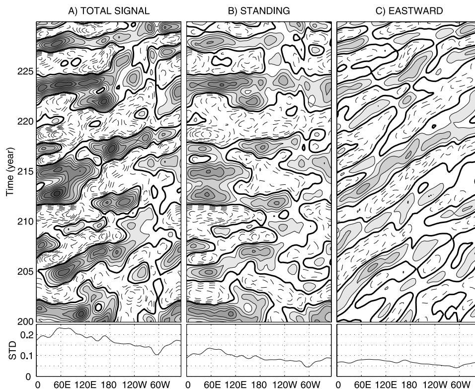
Figure 5. (top) Hovmoller diagram of (a) total, (b) stationary, and (c) eastward components of SST anomalies from CPL simulation for a 30-year section of the integration. Anomalies have been averaged between 41^{\circ}\text{S} and 47^{\circ}\text{S} and band-pass filtered with a 2–20 year band-pass filter. Contours every 0.05 K, with zero contours thick, negative contours dashed, and positive contours shaded. (bottom) SD at each longitude for the entire simulation (K).
