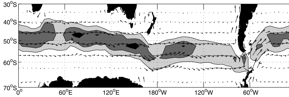
Figure 2. Absolute geostrophic surface current of the model. Light, medium, and heavy gray contours are for current's speed higher than 6, 8, and 10 cm s -1 .
