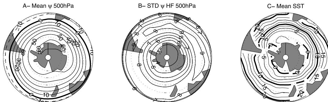
Figure 3. Climatological fields of the CPL simulation. (a) The 500 hPa stream function long-term mean (contours every 10^7 \text{ m s}^{-2} ). (b) SD of 500 hPa stream function fluctuations having period lower than 11 days (contours every 10^6 \text{ m s}^{-2} ). (c) SST long-term mean (contours every 2.5 K).
