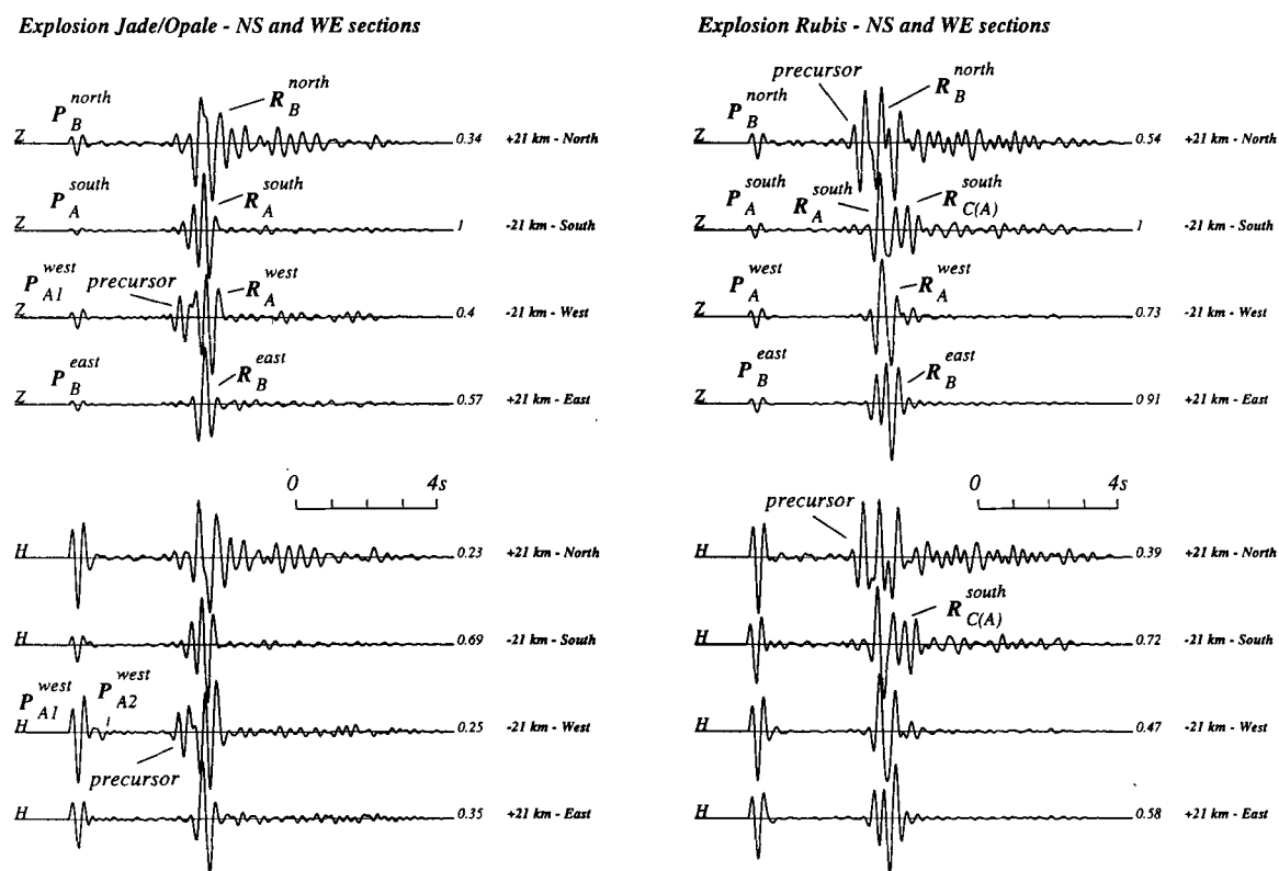
Figure 11. Comparison of the N, S, W and E horizontal and vertical ground velocity components calculated for explosions Jade/Opale and Rubis at 21 km epicentral distance. The relative amplitudes are given for each explosion and component. Source-time function and window duration are those defined in Figs 9 and 10. Phases labelled in Figs 9 and 10 are reported and discussed in the text.
