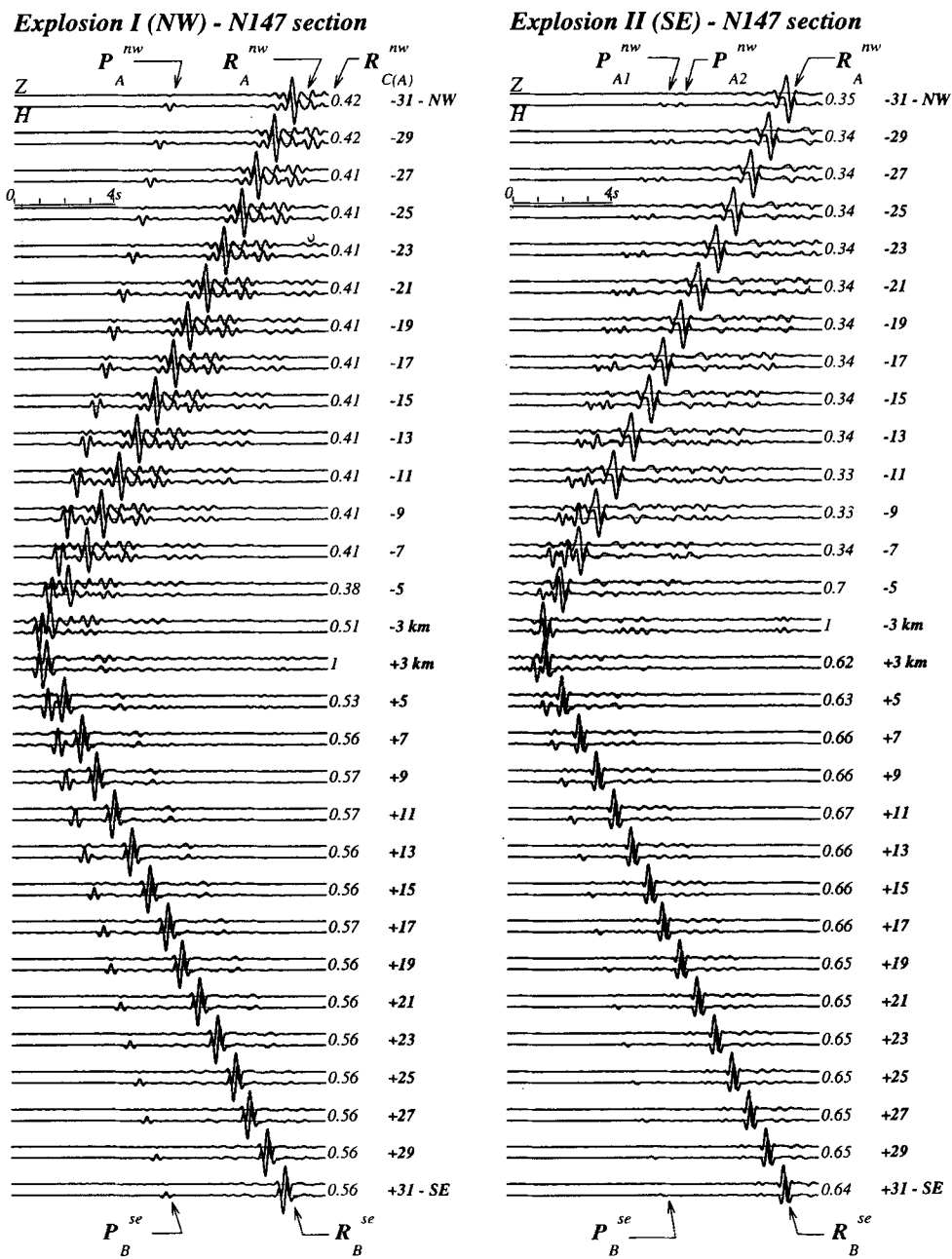
Figure 6. Comparison of ground velocity computed at epicentral distances of 3–31 km from each side of the mountain, for explosions I (left side) and II (right side). The first column in the right side of each stack gives the relative amplitude for each explosion, the second column gives the epicentral distances. See text for explanation. Time duration is 13 s and source time function is a Ricker pulse centred at 3.5 Hz.
