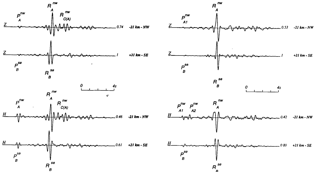
Figure 7. Comparison of the NW and SE horizontal and vertical ground-velocity components recorded for explosions I and II at 21 km epicentral distance. The names of different point phases are given with their significances explained in the text. Relative amplitudes are given for each component and for each detonation point.
