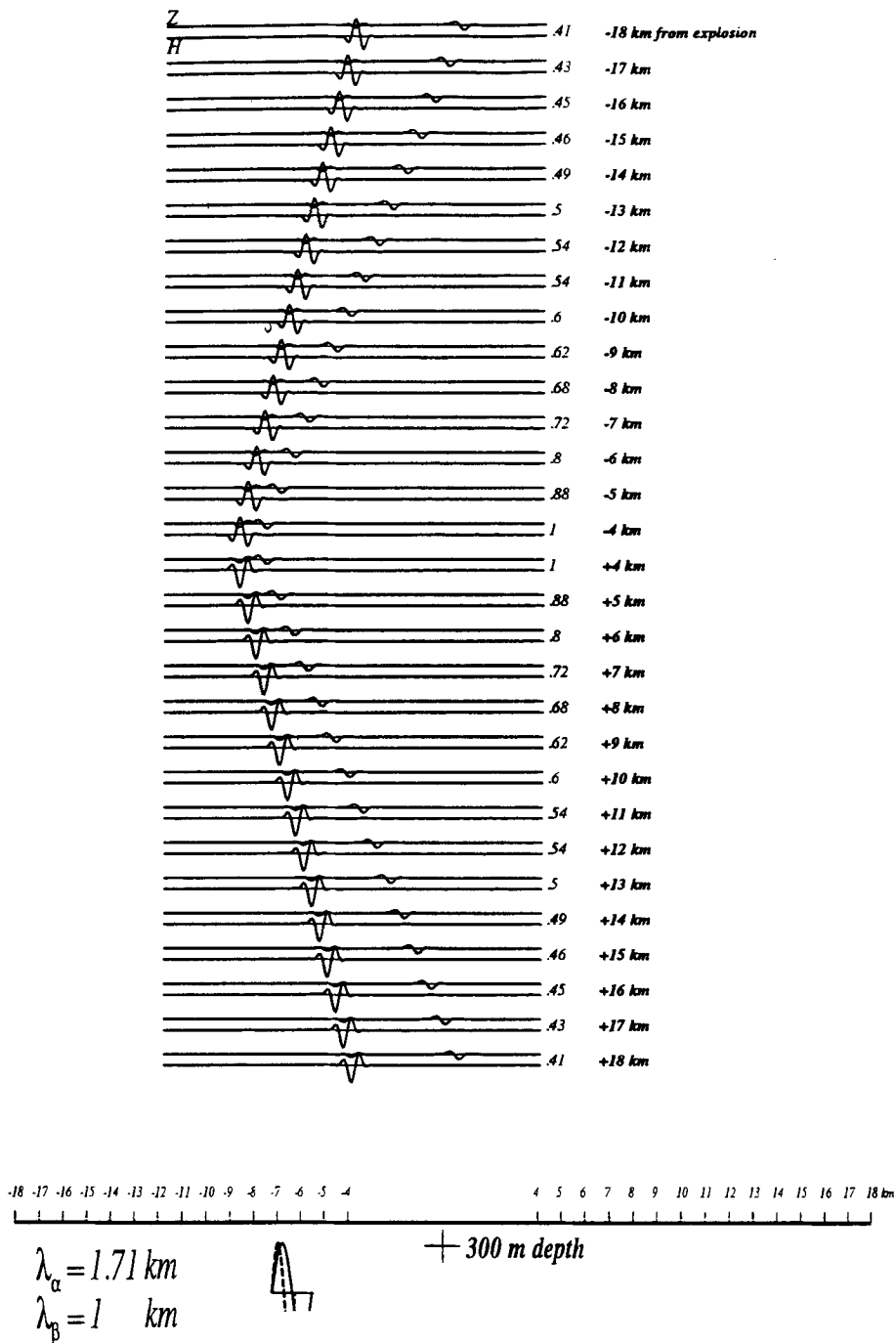
Figure 4. Horizontal (H) and vertical (Z) components of the ground velocity computed for an explosion buried at 300m depth under a flat surface in a homogeneous space. The source is a Ricker pulse centred at 3.5 Hz. The time window is 7.8 s. Receivers are identified by their epicentral distances (from -18 km to +18 km).
