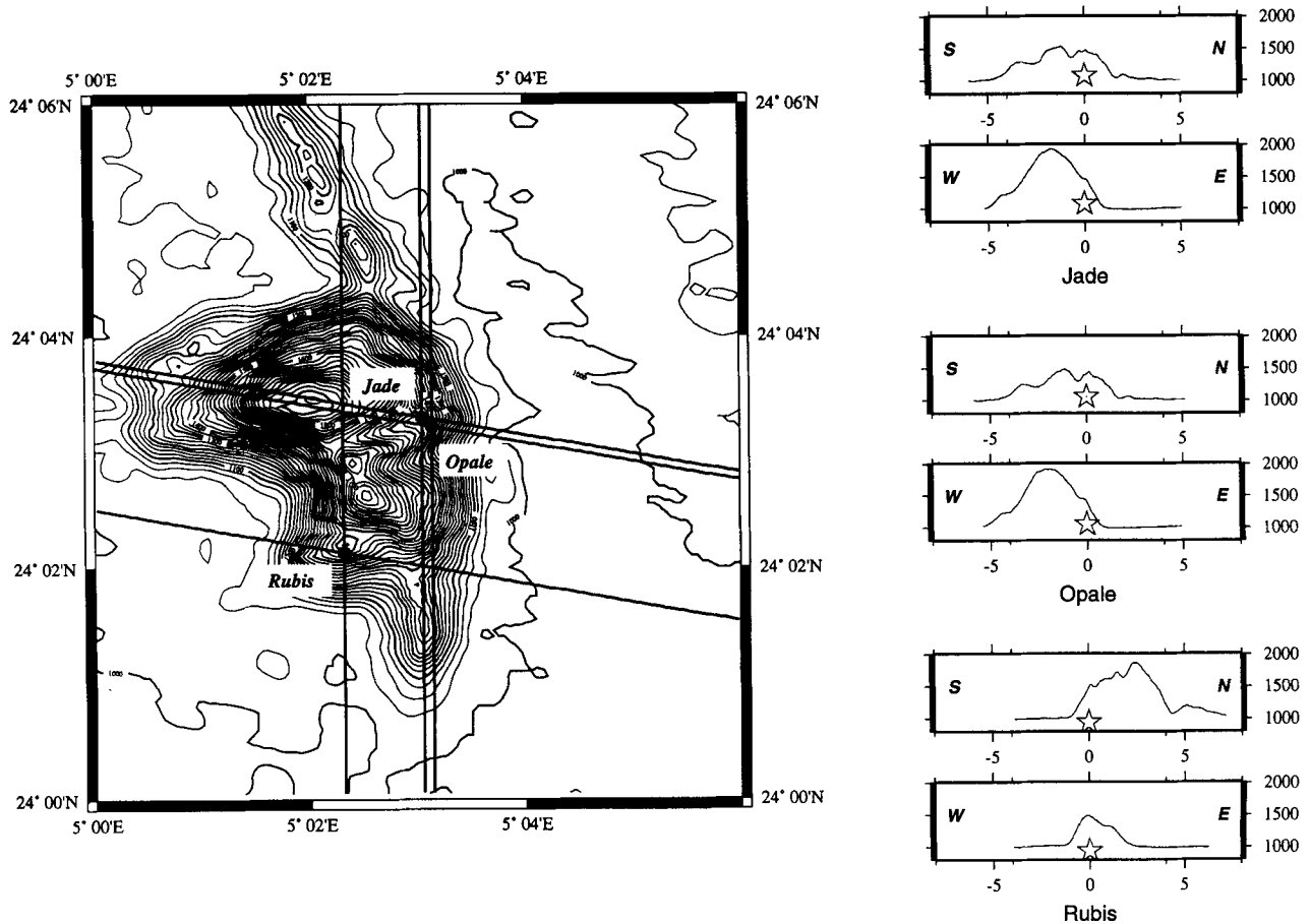
Figure 8. Realistic configuration for Jade, Opale and Rubis. Two 2-D sections (N-S and W-E) are reported on the right side for each detonation point. Elevation and offset from shot are given in metres and in kilometres, respectively.
