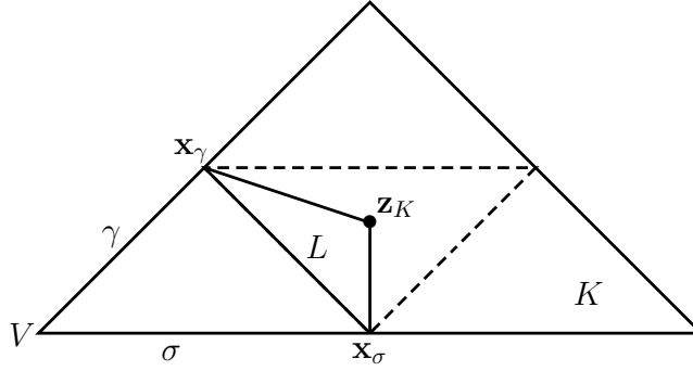
Figure 3: Triangle K \in \mathcal{T}_h and subtriangle L given by two edge midpoints \mathbf{x}_\sigma and \mathbf{x}_\gamma and the point \mathbf{z}_K
