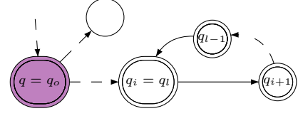
Fig. 6. Principle for tagging persistent states in DFA2S_Per
