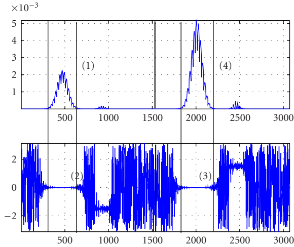
FIGURE 12: Upper plot = modulus of diagonals of blocks (1) and (4) diagonals of the spectral matrix of wave 1 (Figure 8). Bottom plot: angle of blocks (2) and (3) diagonals of the spectral matrix of wave 1 (Figure 8).
