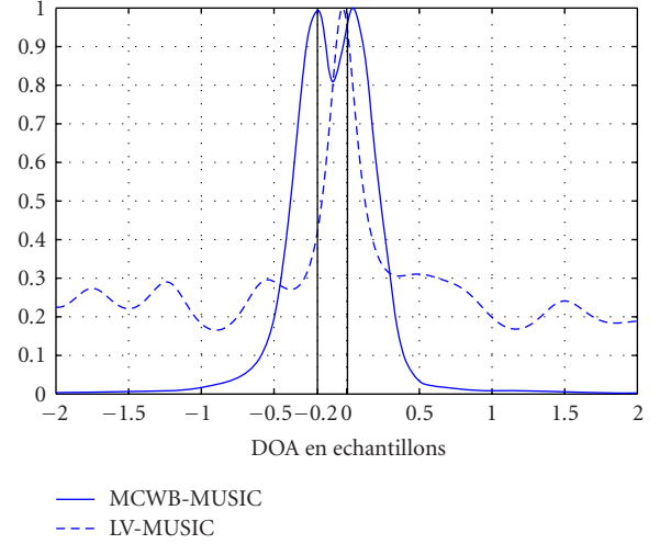
FIGURE 17: Comparison between MW-MUSIC and LV-MUSIC.
