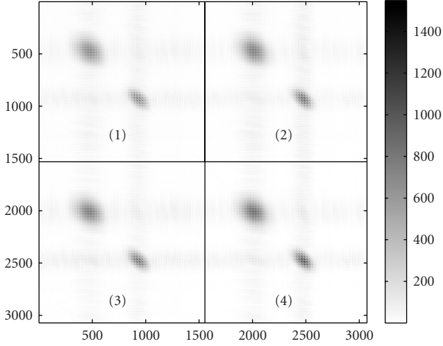
FIGURE 7: Modulus of the Multicomponent Wideband Spectral Matrix of the initial dataset (of size 3072 \times 3072 with 3072 = 24 \times 64 \times 2 ). Compared with Figure 1, block 1 is \underline{\Gamma}_{XX} , block 4 is \underline{\Gamma}_{ZZ} and blocks 2 and 3 are \underline{\Gamma}_{XZ} , \underline{\Gamma}_{ZX} , respectively.
