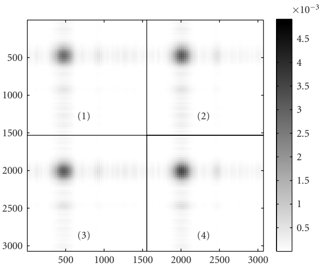
FIGURE 8: Modulus of the multicomponent wideband spectral matrix of the first extracted wave, \underline{\Gamma}_{s,1} .
