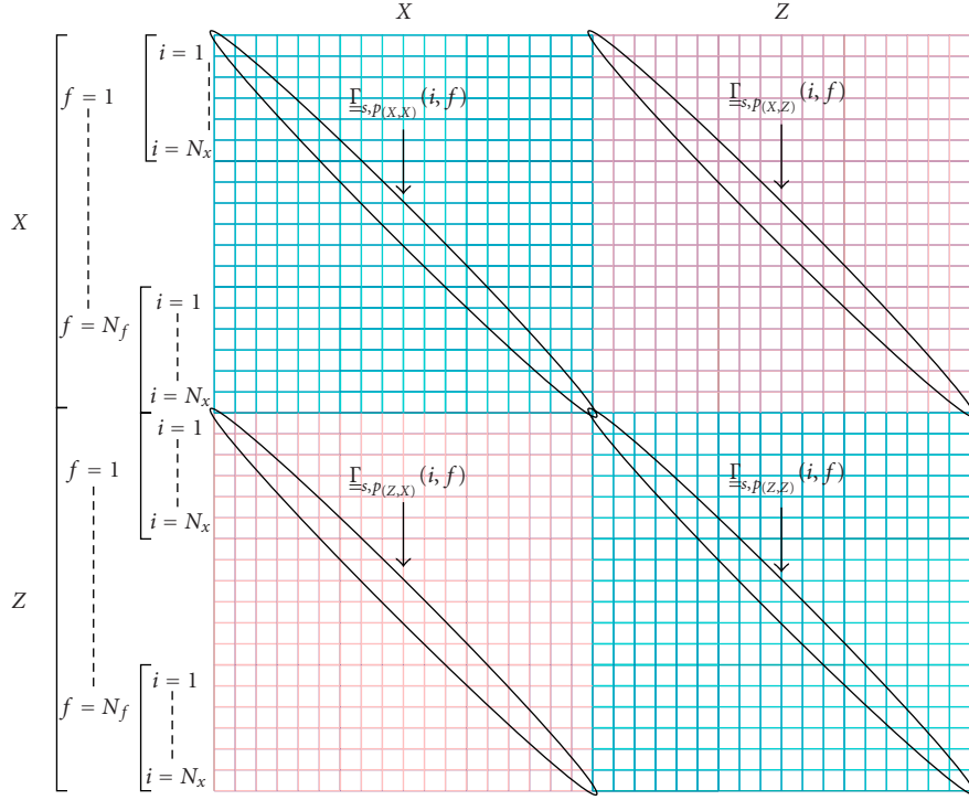
FIGURE 2: Diagram of \underline{\Gamma}_{s,p} , the 2-Component wideband spectral matrix of the wave p .
