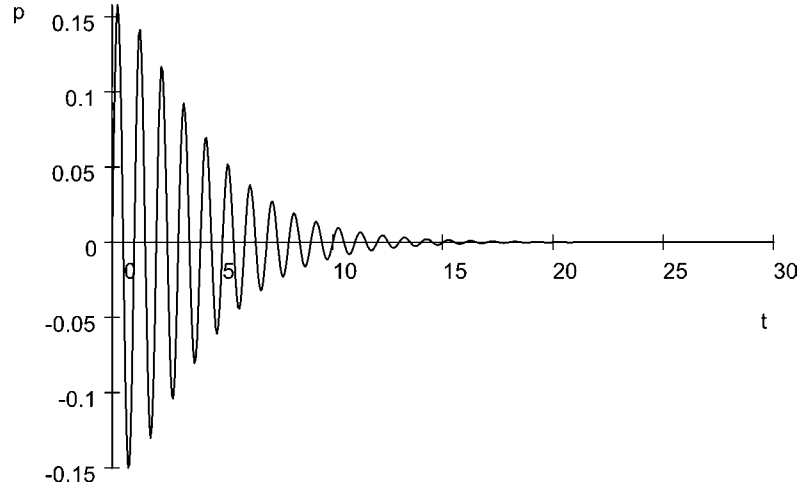
Fig. 6. Time evolution of p_k(t) . A characteristic time equal to the period of free vibrations of the k th mode has been chosen.
