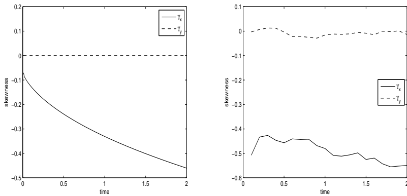
Fig. 10. Experiment 2. Skewness in x and y for the PDE model (left) and for the IBM (right).
