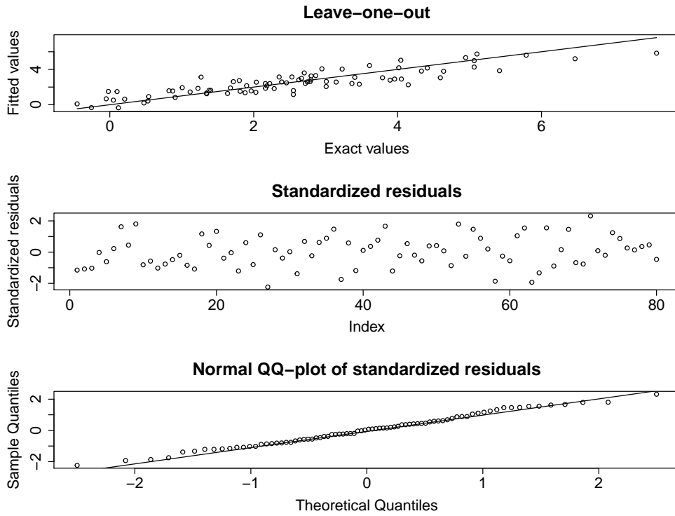
Figure 14: Leave-one-out validation for the 6-d Hartman function.
