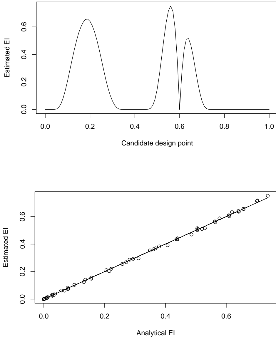
Figure 30: 1-point EI estimated by Monte Carlo (top) and comparison to the previous results obtained with the analytical formula (bottom).
