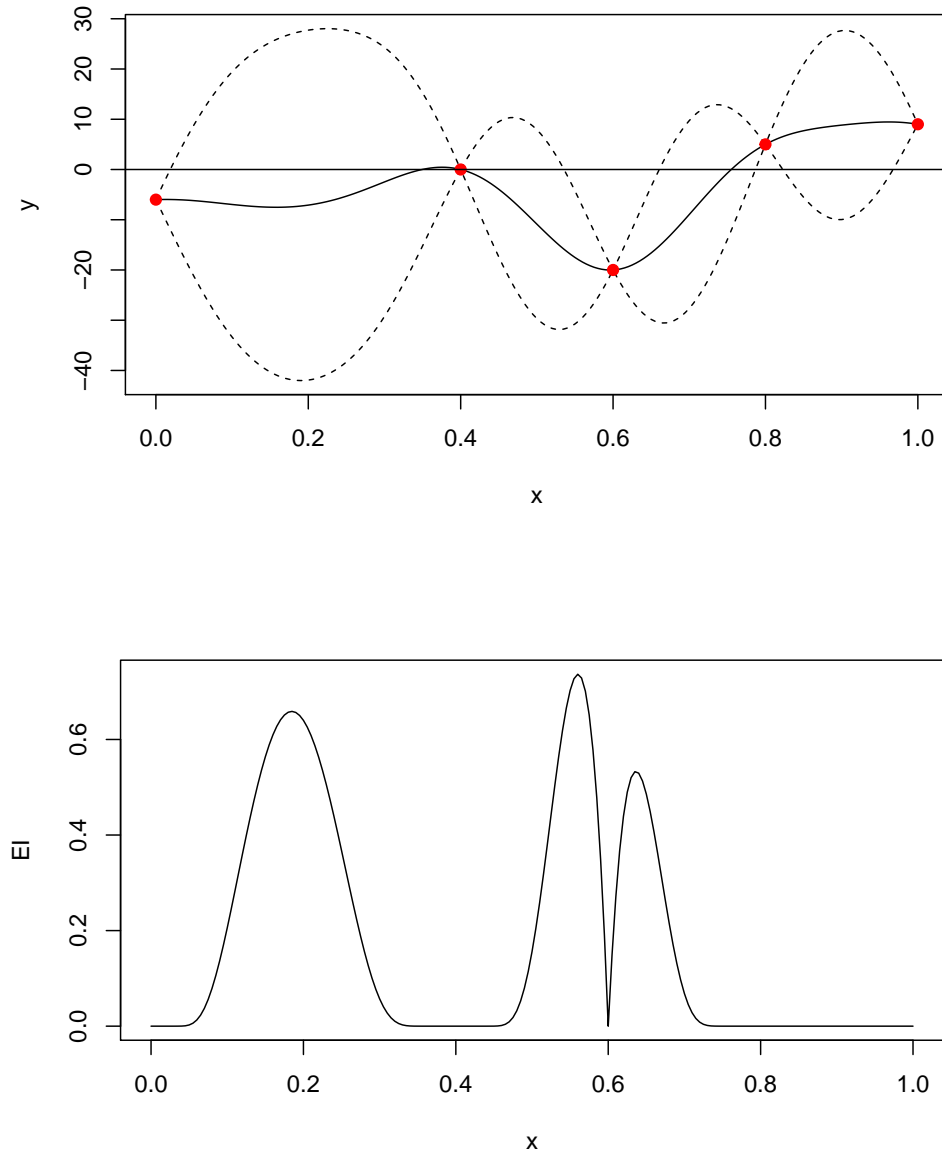
Figure 22: The first 1-dimensional toy example described in this section (top), and its associated EI (bottom).
