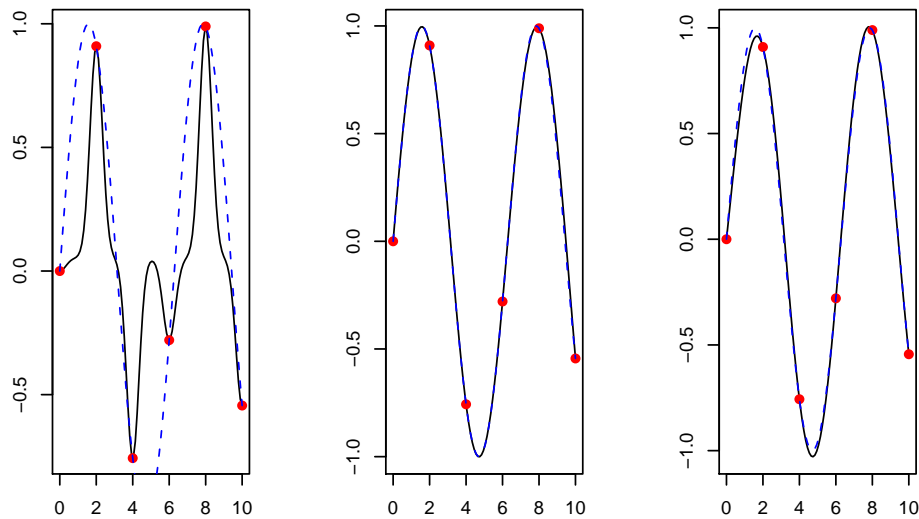
Figure 19: Comparison of three estimation methods for kriging approximation of the sine function, with 6 design points: MLE (left), PMLE with SCAD penalty (middle), MLE constrained by \theta \geq 10/5 (right). The bullets represent the design points, the solid line the Kriging mean and the dotted line the sine function.
