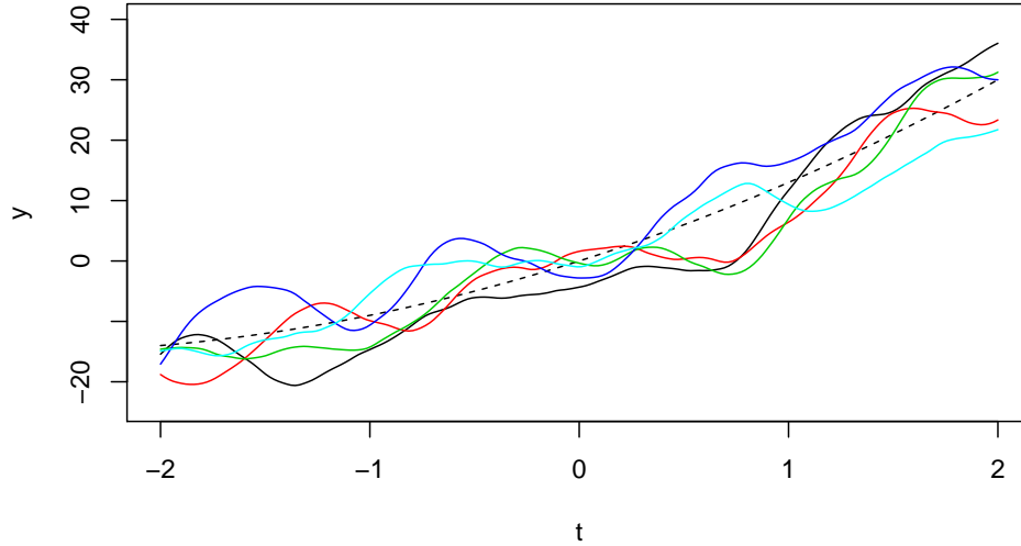
Figure 4: Unconditional simulations of a trended 1-d Gaussian process with Matérn covariance ( \nu = 5/2 ).
