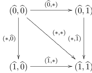
FIGURE 3. The flow \{\hat{0} < \hat{1}\}^2 ((*, *) = (\hat{0}, *) * (*, \hat{1}) = (*, \hat{0}) * (\hat{1}, *))
