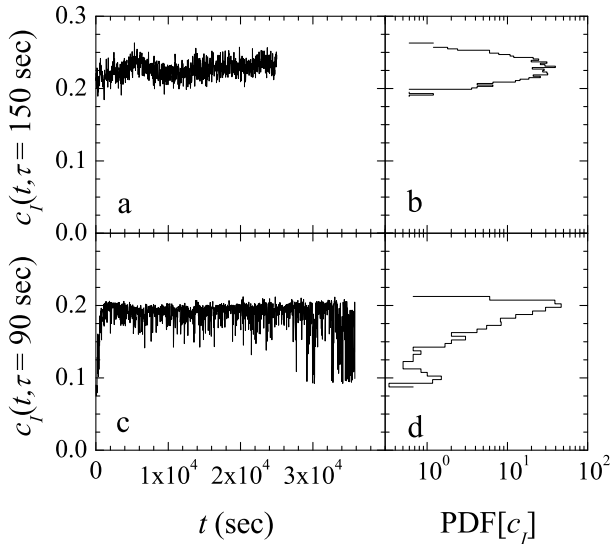
FIG. 3: For a representative ROI, degree of correlation c_I at a fixed delay \tau as a function of time and its PDF for the “artificial skin” in humid (RH = 62%, \tau = 150 sec, panels a and b) and dry (RH = 12%, \tau = 90 sec, panels c and d) atmosphere. Note that the dry sample exhibits large temporal fluctuations.
