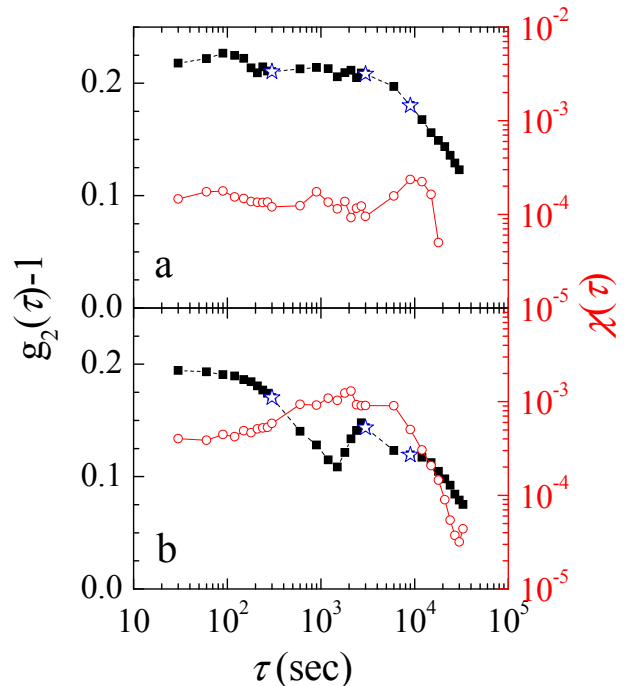
FIG. 2: Intensity time autocorrelation function, g_2 - 1 (left axis and solid black squares), and dynamical susceptibility, \chi (right axis and open circles), for the “artificial skin” sample, as measured in the backscattering configuration schematized in Fig. 1b. a: relative humidity = 62%; b: relative humidity = 12%. Note the enhanced dynamical heterogeneity in dry atmosphere, as shown by the higher values of \chi . The three lags indicated by open stars are those for which the spatial correlation of the dynamics is shown in Fig. 4.
