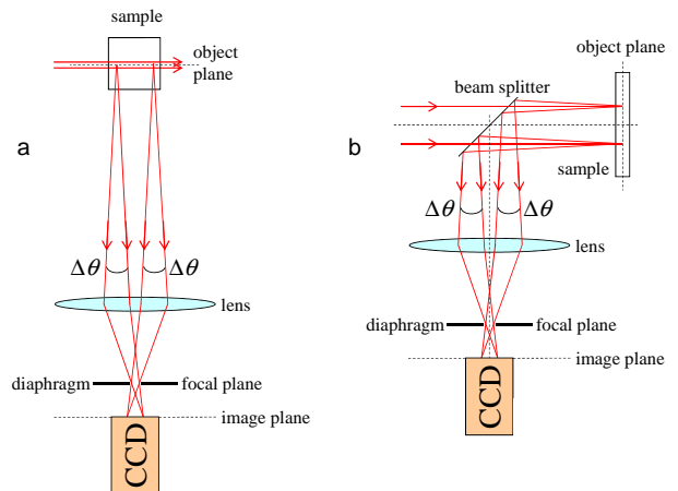
FIG. 1: Scheme of a PCI setup in two different configurations: a) 90^\circ scattering angle; b) backscattering. From Ref. [30] with permission.
