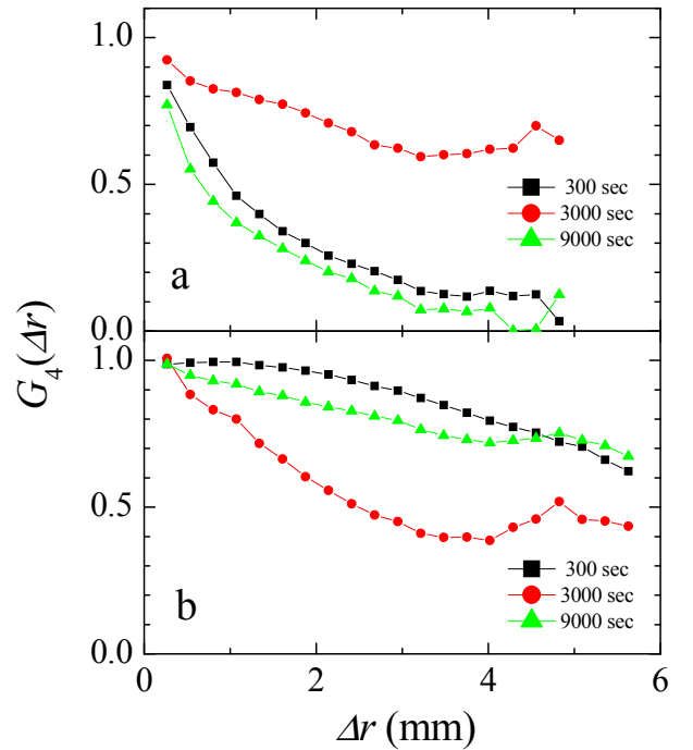
FIG. 4: Spatial correlation of the dynamics, G_4(\Delta r) , for the “artificial skin” samples in humid (RH = 62%, a) and dry (RH = 12%, b) atmosphere. The curves are labeled by the temporal lag at which the dynamics were probed.
