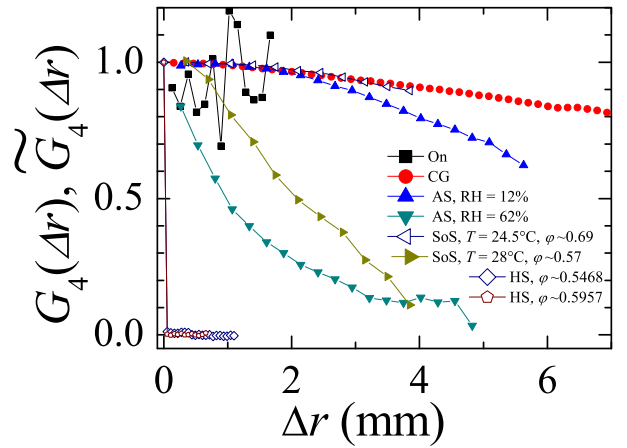
FIG. 5: Spatial correlation of the dynamics for all systems that we have studied except for Laponite, as indicated by the label (On: onion gel; CG: colloidal gel, from Ref. [30]; AS: “artificial skin”, \tau = 300 sec; SoS: soft spheres, from [31]; HS: hard spheres). Data for Laponite are shown in Fig. 6 below. All spatial correlation functions have been normalized according to Eq. (6), except for the hard spheres, for which \widetilde{G}_4 is shown (see Eq. (5)), rather than G_4 .
