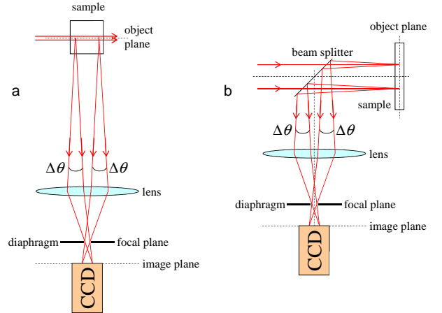
FIG. 1: Scheme of a PCI setup in two different configurations: a) 90^\circ scattering angle; b) backscattering. From Ref. [30] with permission.
