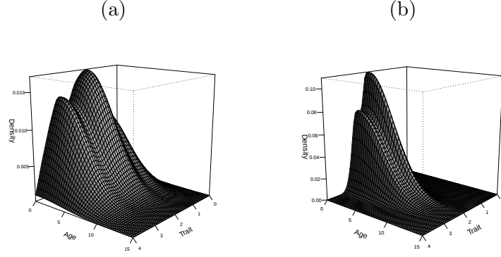
Figure 3: Joint distributions in trait and age for the simulation of Fig. 2. We see that contrarily to Example 1, we do not have here independence of traits and age. (a): \sigma = 1 . (b): \sigma = 0.2
