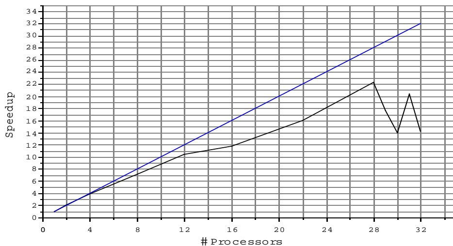
Figure 8: Speedups observed on the Cray T3D
