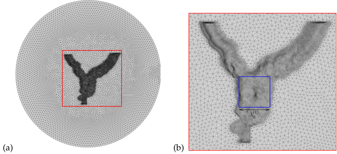
Figure 5: Density of points per S-wavelength in \Omega^{(1)} (a) and close-up on the density of points per \lambda_S^{(1)} on the interface \Gamma_{12} (b), for N = 141,288 and f = 0.6 Hz.
