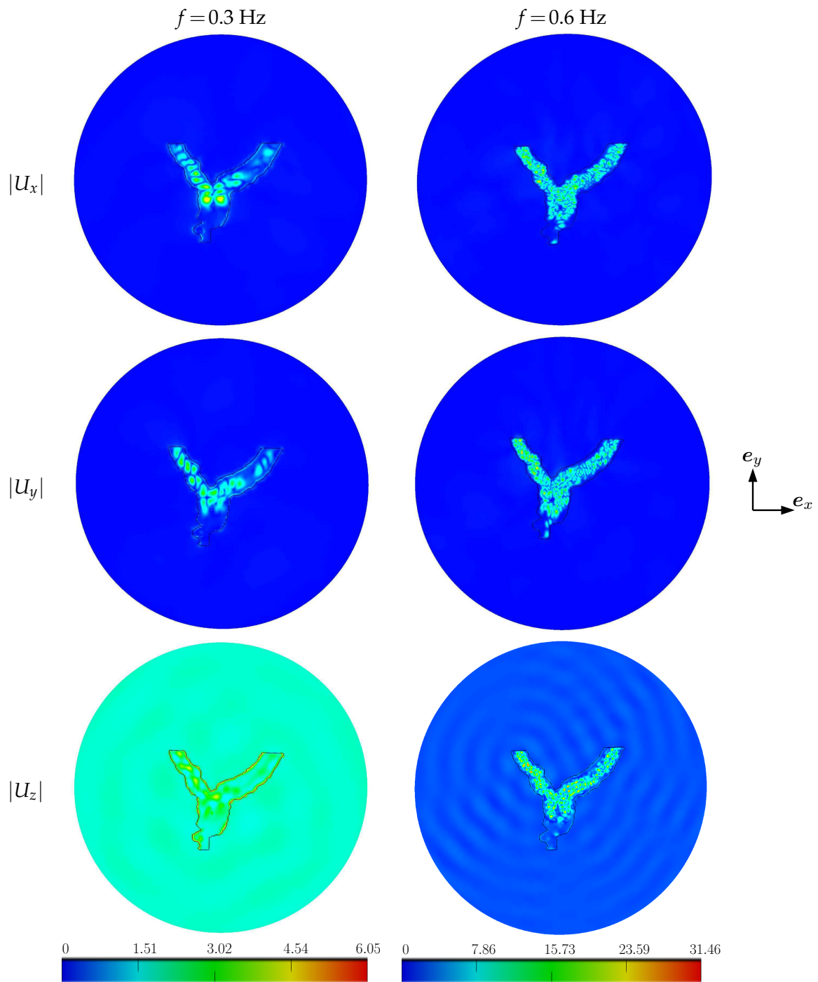
Figure 3: Propagation of a vertical incident plane P-wave in the Alpine valley: modulus of the x- (top), y- (middle) and z- (bottom) components of displacement for frequencies f = 0.3 Hz (left) and f = 0.6 Hz (right).
