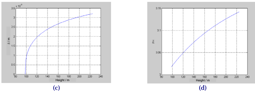
Figure 3: Liquid film thickness (c) and pH (d) along the chimney
