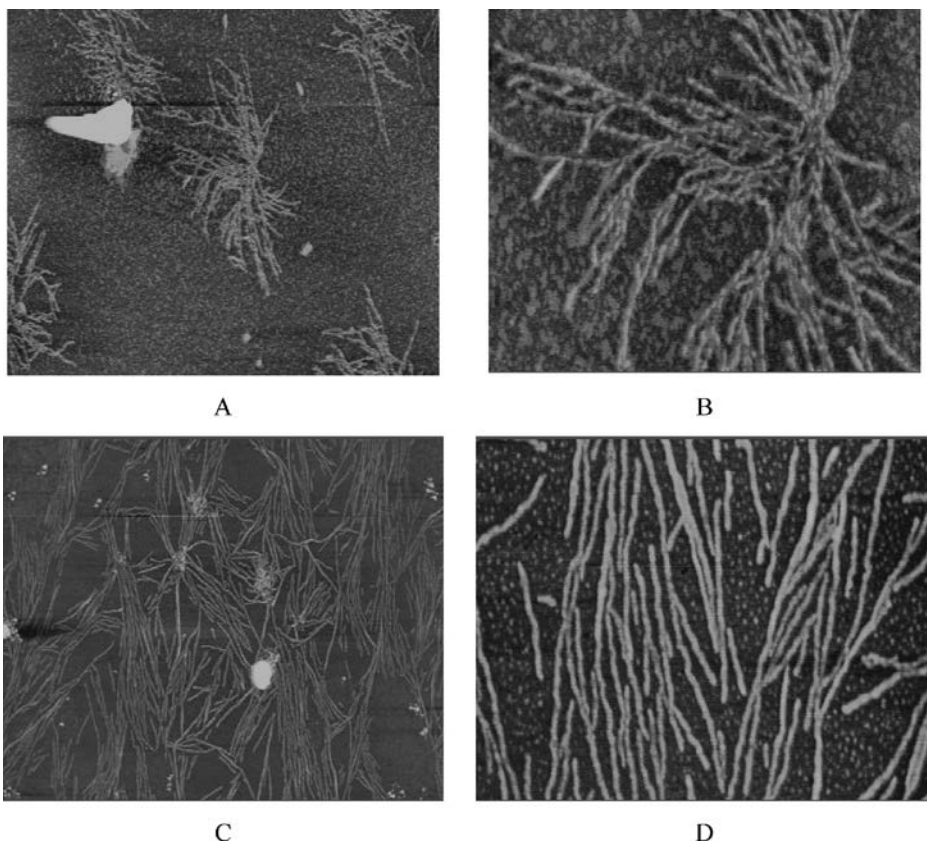
Figure 3. Typical AFM images of (A) PLLA deposited on mica from a 100 \text{ mg} \cdot \text{L}^{-1} solution (scan size is 10 \text{ } \mu\text{m} \times 10 \text{ } \mu\text{m} ); (B) Zoom of the same sample showing the center of nucleation of the aggregate (scan size is 2.5 \text{ } \mu\text{m} \times 2.5 \text{ } \mu\text{m} ); (C) PDLA deposited on mica from a 500 \text{ mg} \text{ L}^{-1} solution (scan size is 10 \text{ } \mu\text{m} \times 10 \text{ } \mu\text{m} ); (D) zoom of the same sample showing that the associated molecules are formed by the connection of the rigid individual macromolecules (scan size is 2.5 \text{ } \mu\text{m} \times 2.5 \text{ } \mu\text{m} ).
