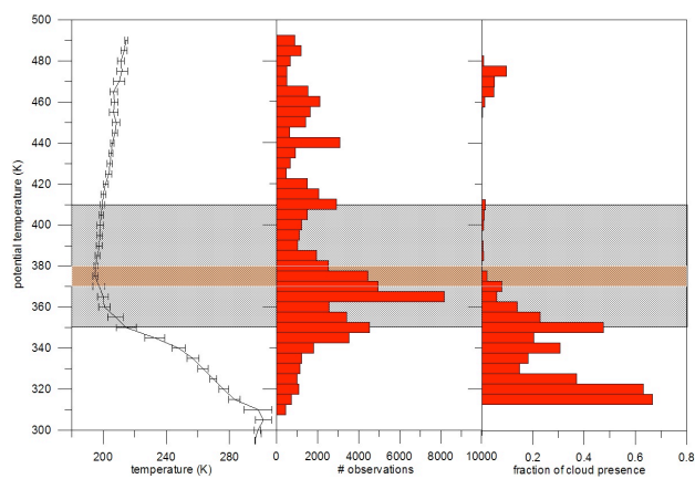
Fig. 2. Left panel: temperature versus potential temperature as measured along the M55 flights between 1–16 August 2006. Only data southward of 17.5° N were used to calculate averages. Bars denote one standard deviation. Middle panel: total number of observations in seconds spent at a given theta level versus potential temperature. Right panel: fraction of observations in cloudy (hazy) air, defined as air masses with Volume Backscatter Ratio >1.2. Grey shading denotes main TTL region and brown shading the tropopause. See text for details.
