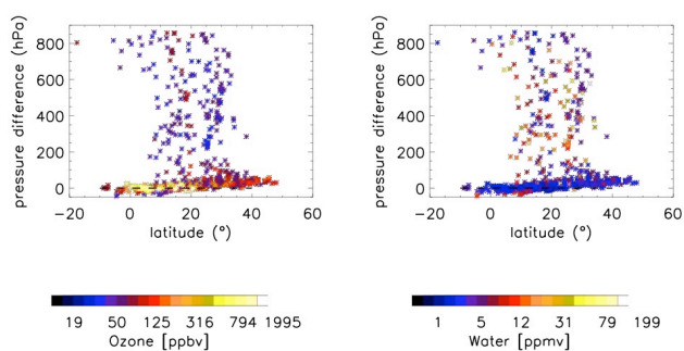
Fig. 6. Scatter plot of the pressure differential versus latitude differential along the back trajectories starting from M55 flight tracks, colour coded in terms of ozone in ppbv (left panel) and water vapour in ppmv (right panel) observed along the flights.
