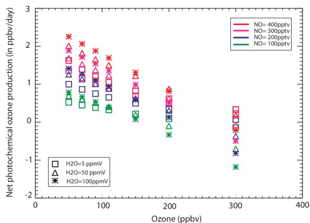
Fig. 13. TTL net photochemical O_3 production rates (ppbv per day) versus initial ozone concentrations (ppbv) as a function of initial H_2O concentrations (ppmv, symbols – see inset) and NO concentrations (pptv, colours as indicated). Results from photochemical model simulations run for 4 days at 150 hPa and initialised with concentrations taken from aircraft observations in the upper troposphere. Net photochemical O_3 production rates are averages over the last 24 h. See text for further details.
