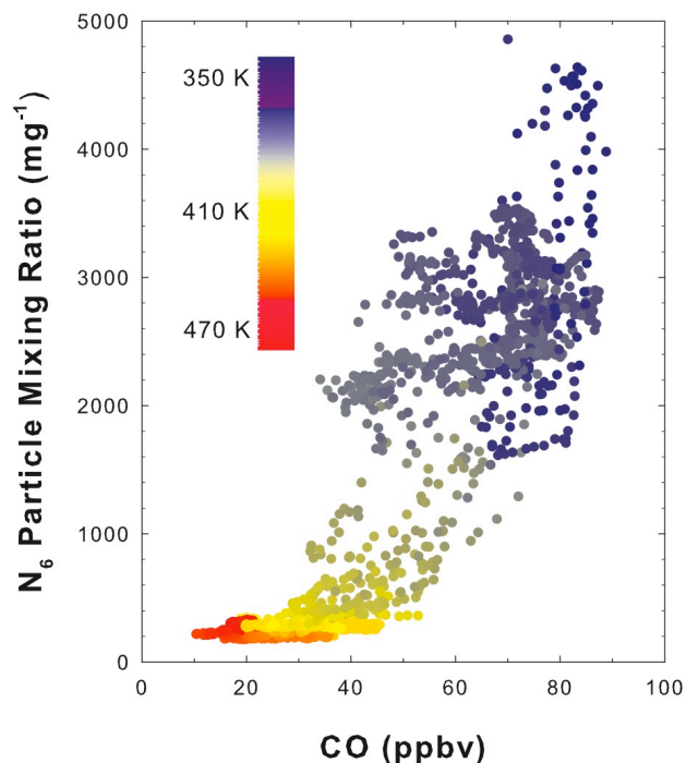
Fig. 11. Scatter plot of CO (ppbv) versus aerosol mass mixing ratio (greater than 6 nm, less than 1\ \mu\text{m} ) (particles per milligram of air) for local M55 flights over West Africa coloured as a function of potential temperature (K). Aerosol nucleation events have been removed (see text for details).
