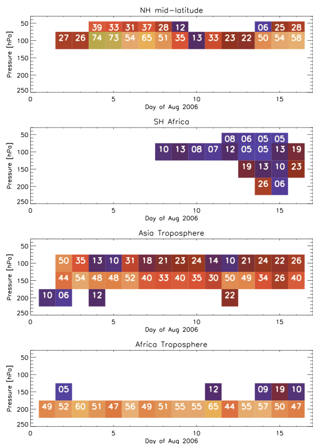
Fig. 4a. Relative contribution of different air mass origin regions (defined in Table 1) based on 10 day back trajectories to air masses arriving over the West African domain (10° E to 40° W and 5 to 25° N) between 1–16 August 2006. Colour codes the percentage of regional influence in terms of fraction of trajectories passing through a particular region (blue = low, red-orange = medium, yellow = high). This value is also expressed numerically in each coloured cell. Note that trajectories can pass through more than one region leading to total fractions of more than 100%.
