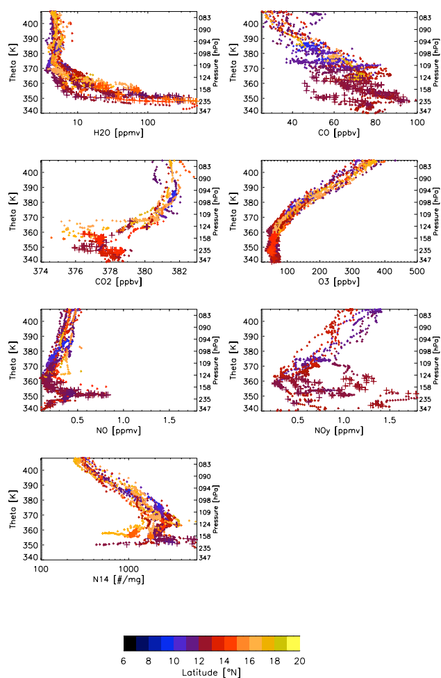
Fig. 10a. Vertical profiles of trace gas concentrations (volume mixing ratio in ppbv or ppmv as appropriate) and aerosol mass mixing ratios (particles per mg air), N_{14} (14 nm < < 1 \mu\text{m} ), for “convective” M55 flights on 7, 8 and 11 August 2006. Profiles are plotted as a function of theta (K) and coloured by latitude where the measurements were made. Crosses indicate points where back trajectories show uplift from below 800 hPa during 10 days before the flight.
