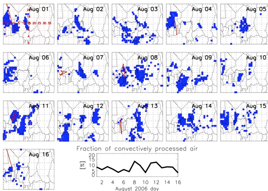
Fig. 8. Daily maps of convective impact at 200 hPa level derived from the percentage of trajectories passing over convective systems diagnosed from MSG cloud tops over the West African domain (blue points, see text for details). M55 flight paths are displayed for the days flights took place. Also shown (inset, bottom right) is an estimate of the fraction of convectively processed air for the West African region. Only grid points where at least 5% of trajectories have been “processed” by convection were used in the calculation of the average.
