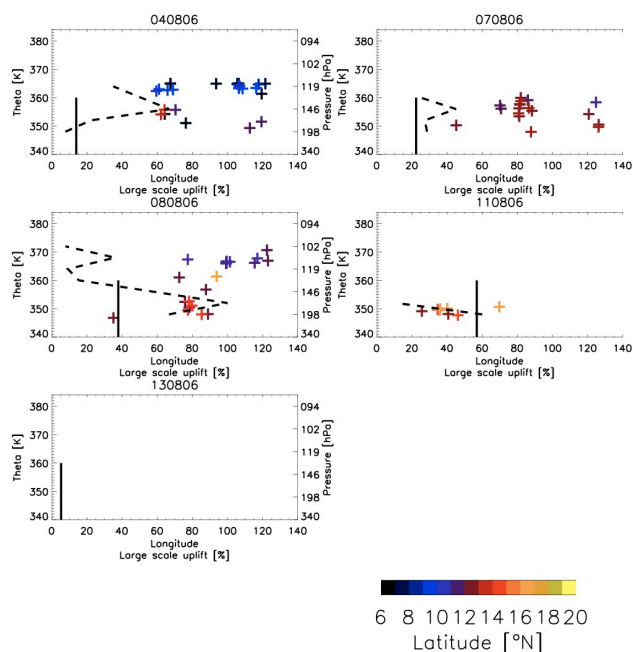
Fig. 9. Fraction of air masses influenced by large-scale convective uplift (%) calculated using 10 day back trajectories arriving along M55 flights in 4 K bins between 340 K and 375 K over West Africa for each local M55 flight (dashed lines). Also shown are average longitudes where air masses arriving along local flights were uplifted irreversibly above 650 hPa coloured by latitude where air masses were sampled by the M55. The average fraction of back trajectories from flight tracks between 350–360 K coinciding with MSG cloud tops (%) are shown as a vertical bar as an indicator of local convective impact (see text for details).
