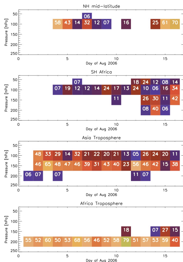
Fig. 4b. Same as Fig. 4a but based on 10 day back trajectories traced back from a sub-domain including the M55 flight tracks (8° E to 5° W and 5 to 15° N).
