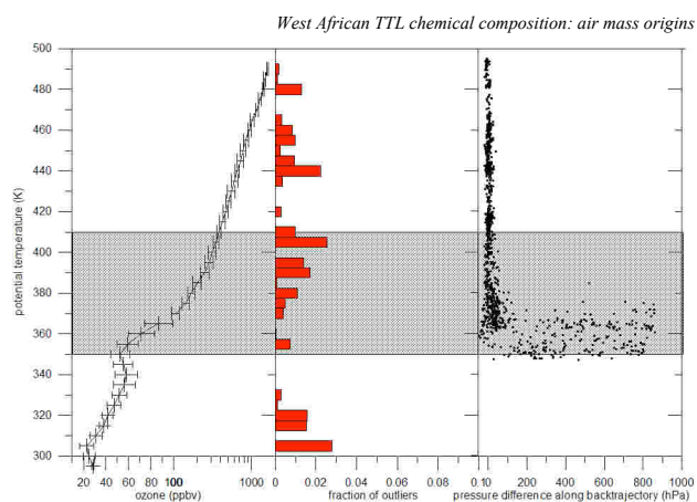
Fig. 12. Leftmost profile, average ozone concentrations (ppbv) using M55 data collected south of 17.5^{\circ} N versus potential temperature (K), bars denote one standard deviation; note the linear ( <100 ppbv)/log ( >100 ppbv) horizontal axis for ozone. Middle bar chart, fraction of ozone data points lying outside three standard deviations from the mean, versus potential temperature; Rightmost panel, pressure difference (hPa) along 10-day back trajectories arriving along M55 flights (south of 17.5^{\circ} N) versus potential temperature (K). Grey shading denotes the main TTL region.
