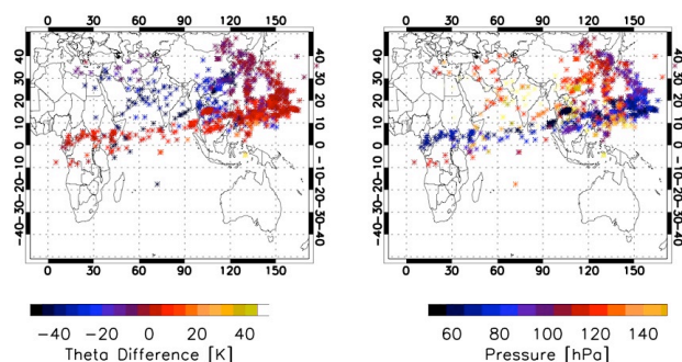
Fig. 5. Starting points of 10-day back trajectories initialised along the M55 flight tracks south of 18^\circ N colour coded in terms of theta variations (K) along the back trajectories (left panel) and pressure at the starting point of the back trajectory, i.e. along the M55 flight path (right panel).
