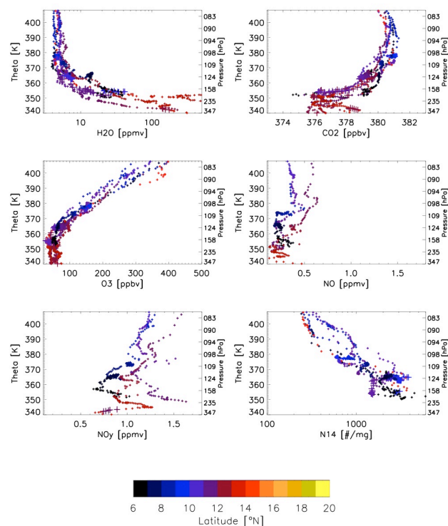
Fig. 10b. Vertical profiles of trace gas concentrations (volume mixing ratio in ppbv or ppmv as appropriate) and aerosol mass mixing ratio (particles per mg air), N_{14} (14 nm to <1\ \mu\text{m} ), for “non-convective” M55 flights on 4 and 13 August 2006. Profiles are plotted as a function of theta (K) and coloured by latitude where the measurements were made. Crosses indicate points where back trajectories show uplift from below 800 hPa during 10 days before the flight.
