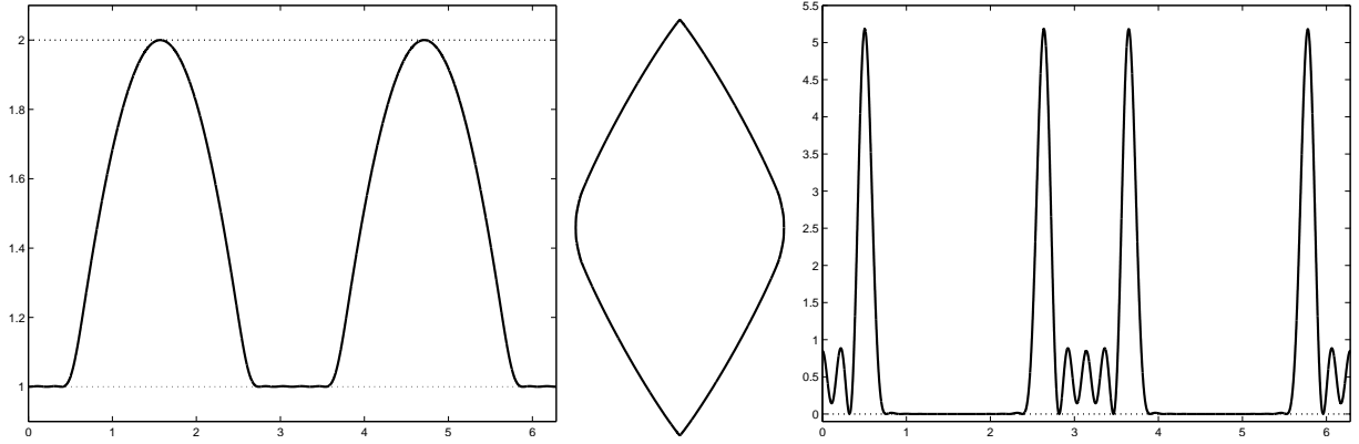
Figure 11: Numerical solution of the perimeter minimization problem for degree 30: width, body and curvature.
