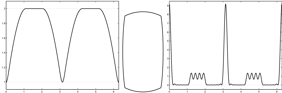
Figure 9: Numerical solution of the perimeter maximization problem for degree 30: width, body and curvature.
