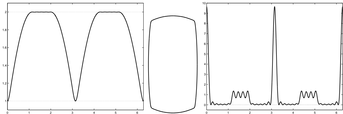
Figure 13: Numerical solution of the area maximization problem for degree 30: width, body and curvature.
