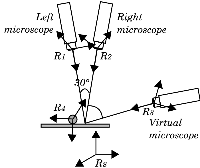
Figure 1: Configuration of the 3-view imaging system. \mathcal{R}_1 , \mathcal{R}_2 , \mathcal{R}_3 , \mathcal{R}_4 and \mathcal{R}_s are the frames of the left, right and novel microscope, an object and the scene, respectively.
