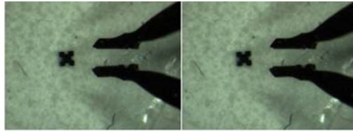
Figure 4: Left and right images used to recovery geometry: the 400 \mu\text{m} \times 400 \mu\text{m} \times 100 \mu\text{m} part is underneath the gripper.
