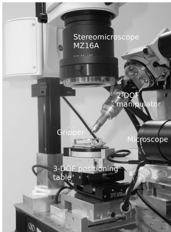
Figure 15: Assembly setup of FEMTO-ST Institute.
