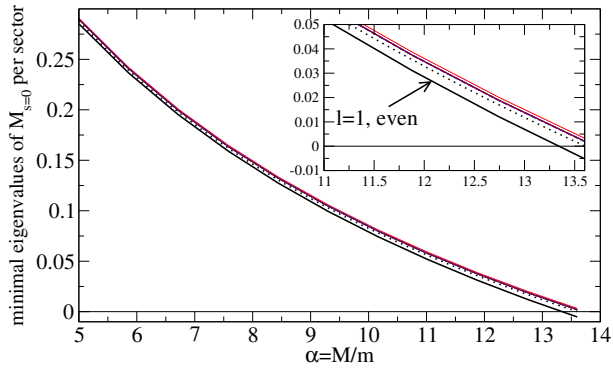
FIG. 1: Minimal eigenvalues of the Hermitian operators M_{s=0} in each sector of fixed parity and angular momentum l , 0 \leq l \leq 6 , as functions of the mass ratio \alpha = M/m . Only the curve for the even sector of l = 1 crosses zero for \alpha < 13.607 , corresponding to the occurrence of a four-body Efimov effect in that sector. The other curves all remain above zero. They strongly overlap and are barely distinguishable at the scale of the figure. The dotted line is the analytical prediction \Lambda(k = 0, \alpha) for the lower border of the continuum in the spectrum of M_{s=0} . The inset is a magnification. In the numerics, x and u were discretized with a step dx = du = 1/10 , and x was truncated to x_{\max} = 20 .
