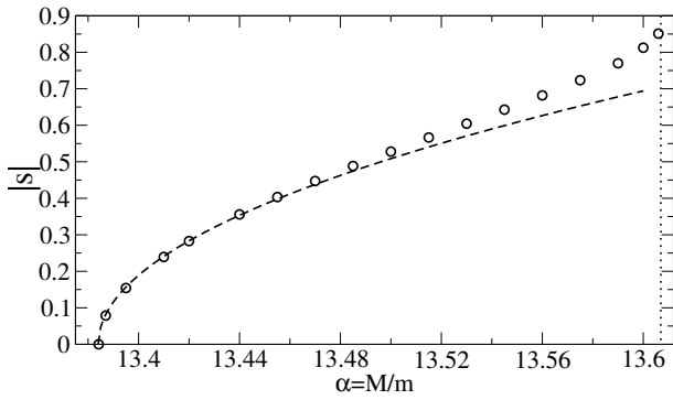
FIG. 2: In the Efimovian channel l = 1 with even parity, modulus of the purely imaginary Efimov exponent s = iS as a function of the mass ratio \alpha = M/m . In the numerics, x_{\max} ranges from 40 to 120, dx = 1/10 , d\theta = \pi/20 . The dashed line results from a linear fit of |s|^2 as a function of \alpha in a vicinity of the critical value \alpha_c(3; 1) , |s|_{\text{fit}}^2 \simeq 2.23 \times (\alpha - \alpha_c) . The vertical dotted line indicates the 2 + 1 critical value \alpha_c(2; 1) .
