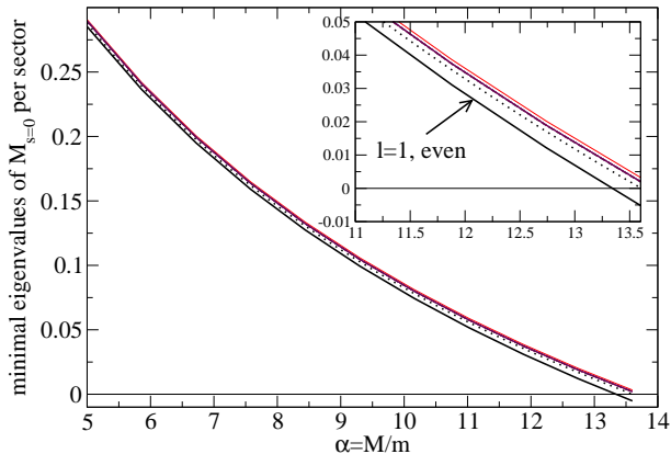
FIG. 1: Minimal eigenvalues of the Hermitian operator M_{s=0} in each sector of fixed parity and angular momentum l , 0 \leq l \leq 6 , as functions of the mass ratio \alpha = M/m . Only the curve for the even sector of l = 1 crosses zero for \alpha < 13.607 , corresponding to the occurrence of a four-body Efimov effect in that sector. The other curves all remain above zero. They strongly overlap and are barely distinguishable at the scale of the figure. The dotted line is the analytical prediction \Lambda(k = 0, \alpha) for the lower border of the continuum in the spectrum of M_{s=0} . The inset is a magnification. In the numerics, x and u were discretized with a step dx = du = 1/10 , and x was truncated to x_{\max} = 20 .
