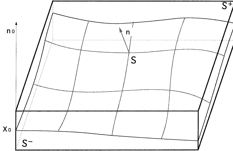
Figure 3. The domain used in the proof of Noll Theorem
