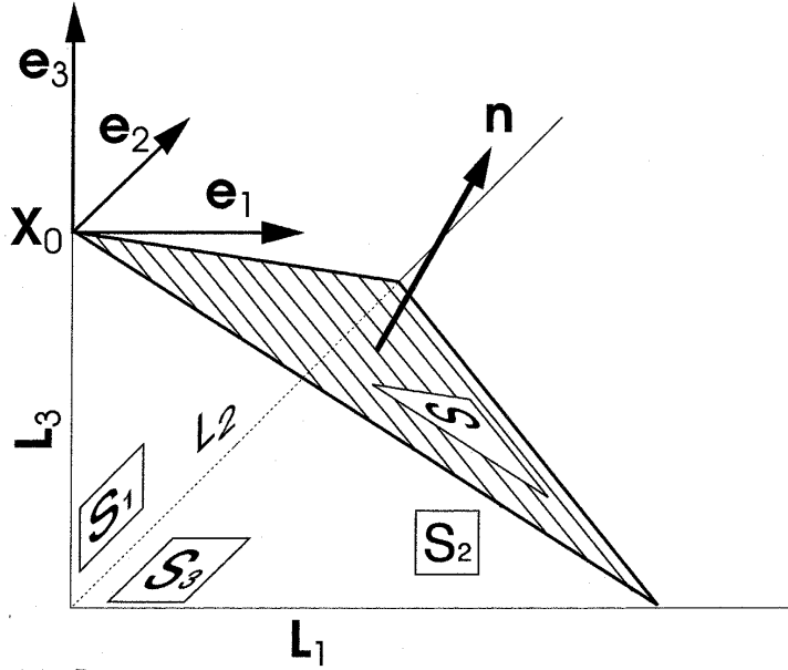
Figure 4. Cauchy's tetrahedron
