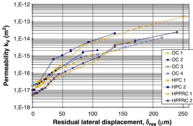
Fig. 15. Gas permeability versus the residual lateral displacement, \delta_{res} .
