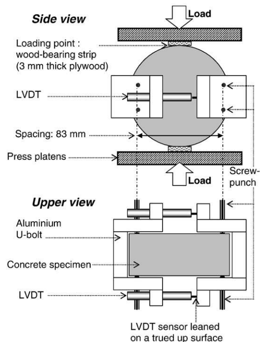
Fig. 1. Lay-out of COD measurement set-up.
