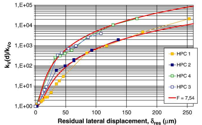
Fig. 23. Adjustment of the model to the relative increases in permeability measured for HPC discs versus the residual lateral displacement, \delta_{res} .
