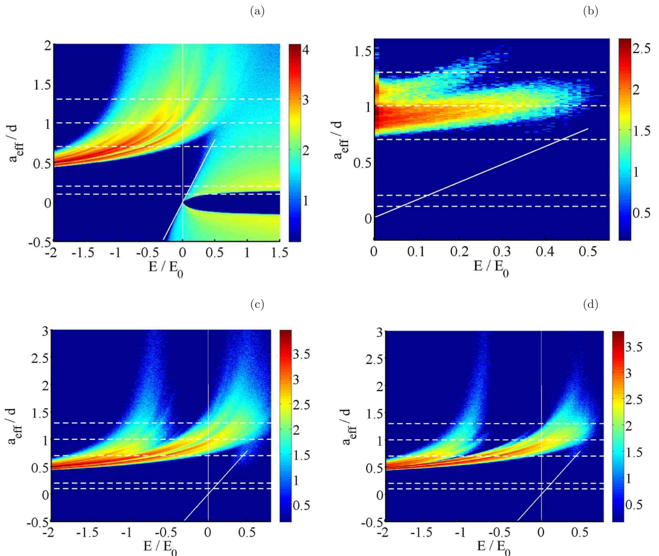
FIG. 7: (Color online) For the 3D system: Density of resonances and bound states per scatterer in the plane (energy E , effective scattering length a_{\text{eff}} ), obtained as explained in subsection IV A. E on the horizontal axis is either the real part of z_{\text{res}} on the positive energy side, or the bound state eigenenergy on the negative energy side. The filling factor is p_{\text{occ}} = 1/10 within a sphere of radius R = 29d , so that the mean number of scatterers is \langle N \rangle \approx 10^4 . The value of E is discretized with a step 0.0025E_0 for both positive and negative values of E , and we use E_0 = \hbar^2/(md^2) as unit of energy. For each value of E one different realization of disorder is used, without imposing any reflection symmetry (see end of subsection III A). A logarithmic scale is used: The color map (see bar on the right) is applied to the quantities \log_{10} \frac{N_{\text{res}}}{N} \frac{E_0 d}{\delta S} , for E > 0 , and \log_{10} \frac{N_{\text{bound}}}{N} \frac{E_0 d}{\delta S} , for E < 0 , where N_{\text{res}} and N_{\text{bound}} are the number of resonances and bound states respectively, within each rectangular bin of area \delta S = \delta E \delta a_{\text{eff}} ( \delta E = 0.01E_0 and \delta a_{\text{eff}} = 0.007d , for both positive and negative values of E ). The plotted quantity is then \simeq \log_{10}(1.4N_{\text{res}}) , and \simeq \log_{10}(1.4N_{\text{bound}}) , respectively. The horizontal dashed lines correspond to the values of a_{\text{eff}}/d \in \{0.1, 0.2, 0.7, 1, 1.3\} used in Fig. 4. The oblique solid line is the border of the energy gap E = \rho g_{\text{eff}} predicted by the mean field theory (see Eq.(18) with \kappa_{\text{mf}} = 0 ). (a) No selection is applied to the resonances ( E > 0 ). As explained in the text, most of the displayed resonances (the ones with too large a width) are not expected to be meaningful. (b) Restricting to E > 0 , only the resonances with a width \Gamma < \Gamma_{\text{max}} = 10^{-6}E_0/\hbar are kept in the density of resonances. The value of \Gamma_{\text{max}} is essentially infinite with respect to the duration of typical experiments: For a matter wave of ^{87}\text{Rb} atoms and an optical lattice with d = 0.4\mu\text{m} , as in [11], one has indeed 1/\Gamma_{\text{max}} \simeq 200 seconds. (c) Only the resonances and bound states corresponding to a small enough participation volume V_p are kept in the density [ V_p^{1/3}/d < 6.5 , see Fig.9a and c]. (d) Only the resonances and bound states corresponding to a small enough r.m.s. size \sigma in real space are kept in the density ( \sigma/d < 4.2 , see Fig.9b and d).
