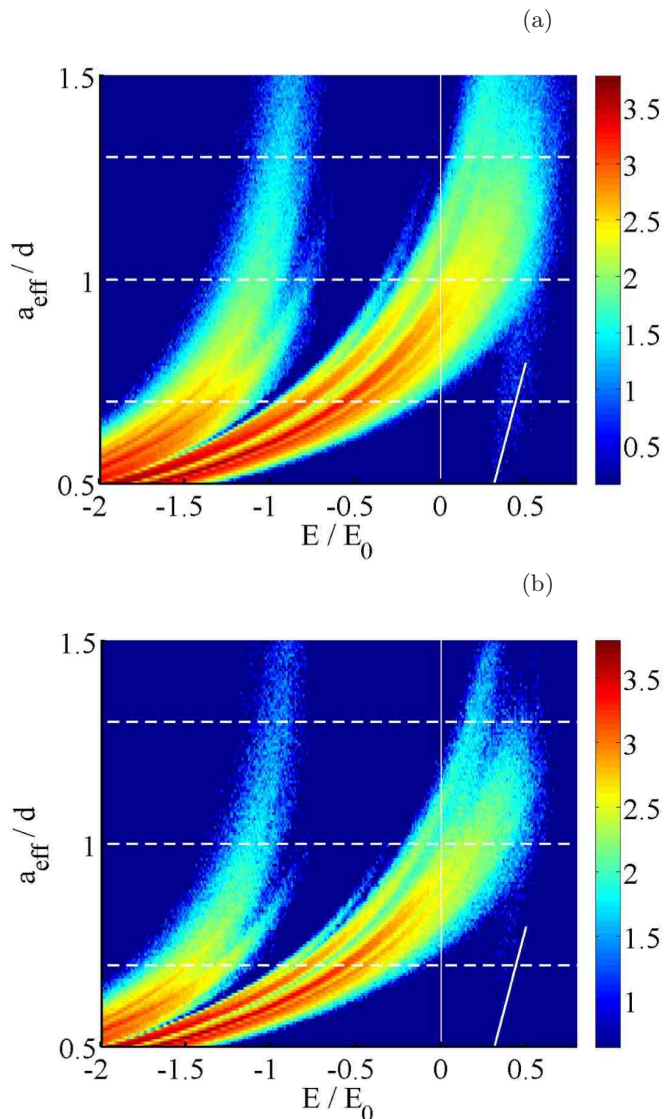
FIG. 10: (Color online) For the 3D system: Finite size effect on the density of localized states. (a) Zoom of the figure 7d, which shows the density of resonances and bound states per scatterer in the plane (E, a_{\text{eff}}) having a r.m.s. size in real space \sigma < 4.2d . We recall that there are N \simeq 10^4 scatterers in a sphere of radius R = 29d . (b) Same as (a), with an additional filtering: we keep only bound states and resonances having their maximum |D_i| at a distance less than R' = 20d from the origin (in the normalization, we considered the number of atoms N' \simeq 3.3 \times 10^3 in the sphere of radius R' ).
