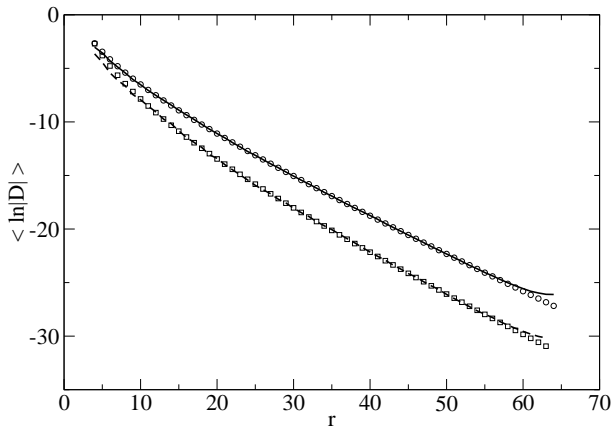
FIG. 3: For the 3D system: Coarse grained histogram \langle \ln |D| \rangle as a function of the distance from the source, for two different kinds of disorder. The first kind of disorder (solid line) is obtained by a random filling of the cubic lattice inside the sphere of radius R = 70d . A second kind of disorder (dashed line) is obtained first by a random filling of the cubic lattice inside only one sector ( 1/8 ) of the sphere, x > 0, y > 0, z > 0 , and then by filling the remaining seven sectors by reflecting the positions in the first sector with respect to planes x = 0, y = 0, z = 0 . The average is taken over 50 realizations of disorder. The filling factor is p_{\text{occ}} = 1/10 , the effective scattering length is a_{\text{eff}} = d and the energy of the emitting source is E = \hbar^2 k^2 / 2m with kd = 0.1 . The circles represent, for the two kinds of disorder, the fit of the histogram on the interval 10d < r < 55d to extract the Lyapunov exponent \kappa with the first method [see Eq. (10)]. We obtain ( \kappa d = 0.31, \alpha = 2.2 ), and ( \kappa d = 0.31, \alpha = 3.6 ), for the first and second kind of disorder, respectively. The Lyapunov exponents appear to be identical, so that one can use the second kind of disorder to calculate \kappa with a substantial gain in the computational effort (a factor 64 on the memory size and a factor 512 in the CPU time).
