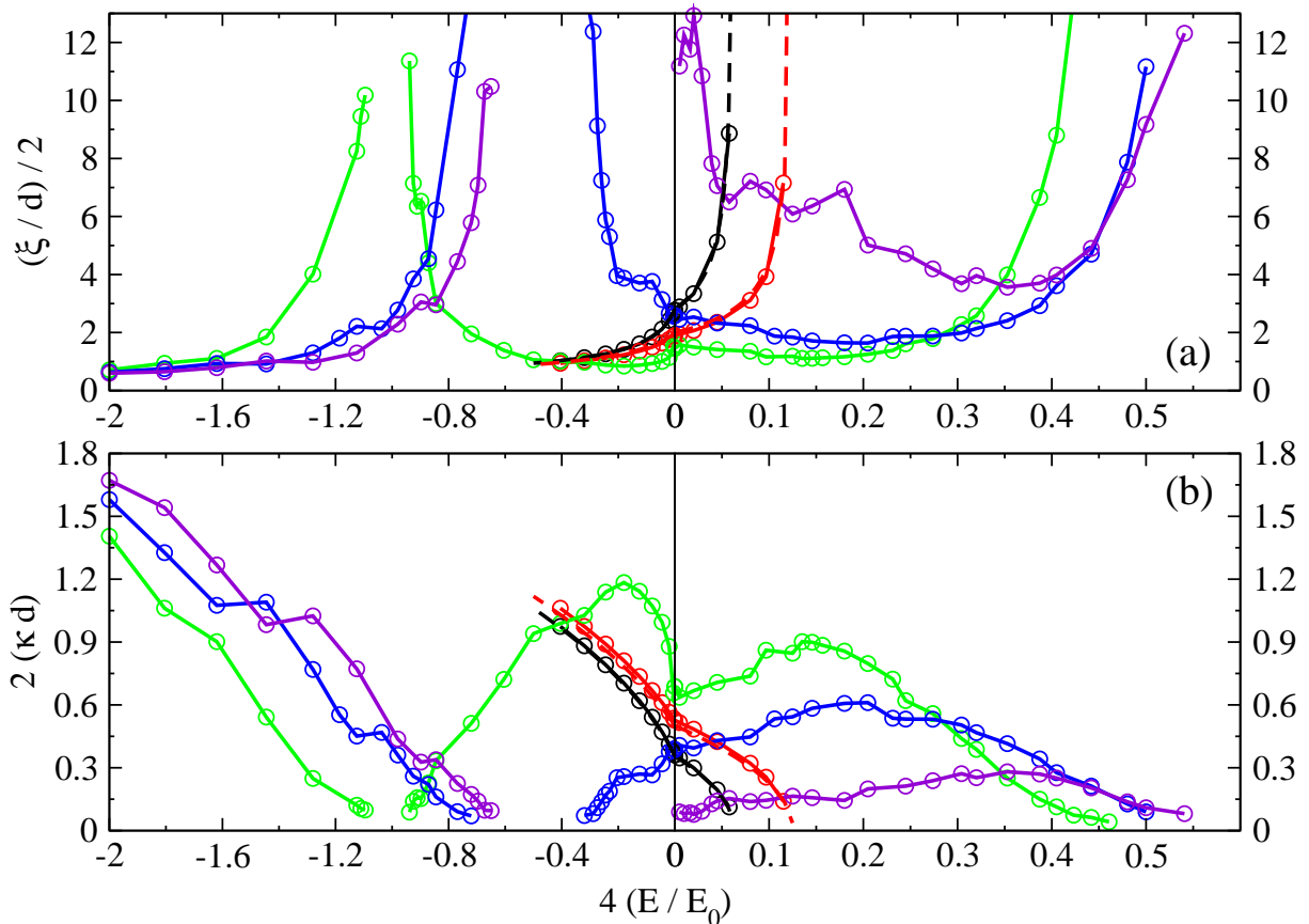
FIG. 5: (Color online) The same as Fig. 4, except that: The value of p_{\text{occ}} is 1/80 , the radius is R = 140d (corresponding to a mean number of scatterers \langle N \rangle \approx 1.4 \times 10^5 ), and a_{\text{eff}} is rescaled to have the same values of \rho^{1/3} a_{\text{eff}} as in Fig. 4, where \rho = p_{\text{occ}}/d^3 is the mean density of scatterers. Since p_{\text{occ}}^{1/3} is two times smaller as compared to Fig. 4, we have a_{\text{eff}} = 2 \times 0.1d (black solid line), a_{\text{eff}} = 2 \times 0.2d (red solid line), a_{\text{eff}} = 2 \times 0.7d (green solid line), a_{\text{eff}} = 2 \times d (blue solid line), a_{\text{eff}} = 2 \times 1.3d (violet solid line). In (a), for 4(E/E_0) = -1.2 , one has a_{\text{eff}}/d = 2 \times 1.3, 2 \times 1, 2 \times 0.7 from bottom to top, and for 4(E/E_0) = 0.2 , one has a_{\text{eff}}/d = 2 \times 0.7, 2 \times 1, 2 \times 1.3 from bottom to top. The axes are rescaled accordingly, to allow a direct comparison with the results of Fig. 4. The number of realizations of disorder is equal to 100 for all points.
