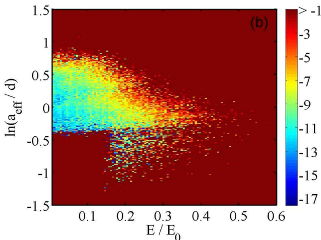
FIG. 18: (Color online) For the 2D system: Width \Gamma of the resonances as a function of the energy E and the logarithm of the effective scattering length \ln(a_{\text{eff}}/d) [see Eqs. (24) and (27), applied to the eigenvalues m_i^\infty(E) of the matrix M_\infty of Eq.(41)]. The physical parameters are the same as in Fig. 14. The plane (E, \ln(a_{\text{eff}}/d)) is decomposed in rectangular bins of widths \delta E and \delta \ln(a_{\text{eff}}/d) . The color map (see bar on the right) is applied to the quantity \log_{10} \hbar \langle \Gamma \rangle / E_0 where \langle \Gamma \rangle is the mean value of \Gamma for the resonances within a given bin. The resonances are filtered in (a) over the participation volume as in Fig. 14c and in (b) over the r.m.s. size \sigma as in Fig. 14d. In (a) one has \delta E = 0.019E_0 and \delta \ln(a_{\text{eff}}/d) = 0.027 , and in (b) one has \delta E = 0.011E_0 and \delta \ln(a_{\text{eff}}/d) = 0.024 .
