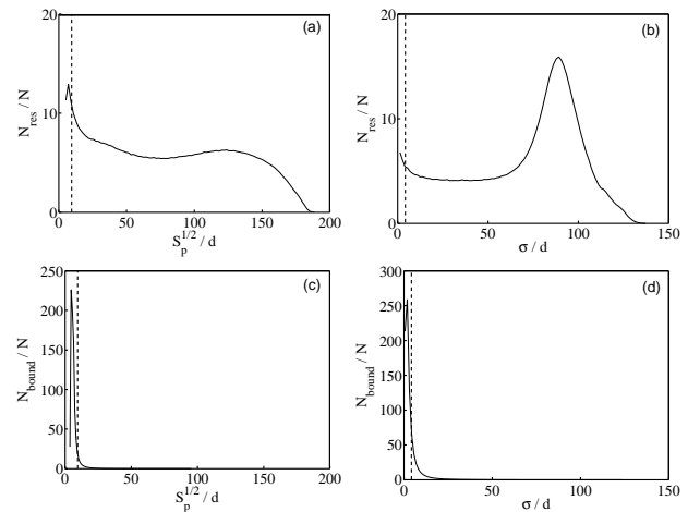
FIG. 17: For the 2D system: For all the resonances with E_{\text{res}}/E_0 \in (0, 2) and \ln(a_{\text{eff}}/d) \in (-3, 3) , and for all the bound states with E/E_0 \in (-2, 0) and \ln(a_{\text{eff}}/d) \in (-3, 3) , the figures show an histogram giving the number of resonances (in (a) and (b)) and bound states (in (c) and (d)) per scatterer (the number of scatterers is N = 7 \times 10^3 ) as a function of: in (a) and (c), the square root of the participation surface defined in Eq.(44); in (b) and (d), the r.m.s. size in real space defined by the 2D version of Eq.(31). The bin size is \sim 0.6d for (a), \sim 1.37d for (b), \sim 0.3d for (c), and \sim 1.37d for (d). The parameters are the same as in Fig. 14a. The dashed vertical lines are the values S_p^{1/2}/d \simeq 9.5 and \sigma/d \simeq 4.2 used in Fig. 14c and Fig. 14d to select the bound states and resonances that are spatially localized and to filter out the bound states and resonances that are weakly localized.
