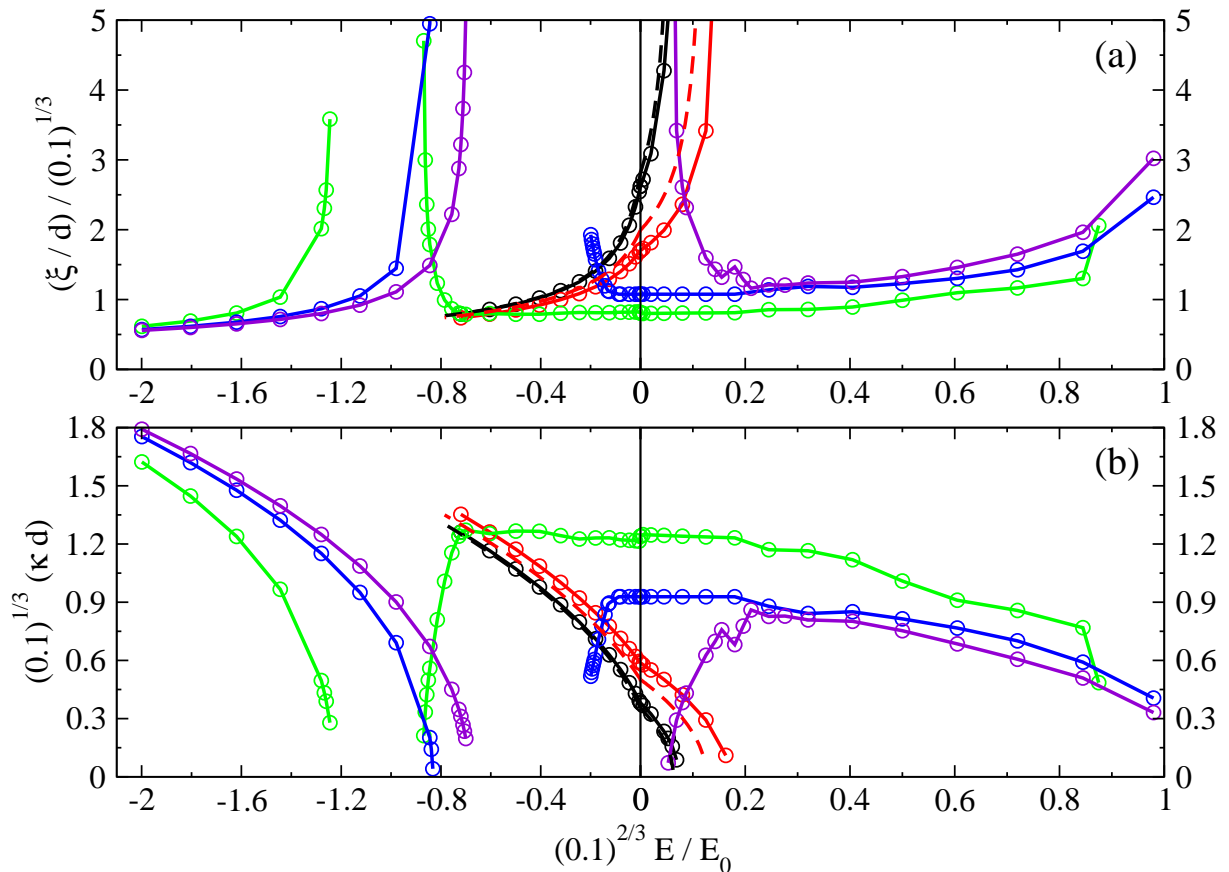
FIG. 6: (Color online) The same as Fig. 4, except that: The value of p_{\text{occ}} is 1 (there is no disorder, since all the lattice sites within the sphere of radius R = 30d are occupied by the scatterers, which leads to N \approx 1.1 \times 10^5 [21]), and a_{\text{eff}} is rescaled to have the same values of \rho^{1/3} a_{\text{eff}} as in Fig. 4, where \rho = p_{\text{occ}}/d^3 is the mean density of scatterers. Since p_{\text{occ}}^{1/3} is (0.1)^{1/3} times smaller as compared to Fig. 4, we have a_{\text{eff}} = (0.1)^{1/3} \times 0.1d (black solid line), a_{\text{eff}} = (0.1)^{1/3} \times 0.2d (red solid line), a_{\text{eff}} = (0.1)^{1/3} \times 0.7d (green solid line), a_{\text{eff}} = (0.1)^{1/3} \times d (blue solid line), a_{\text{eff}} = (0.1)^{1/3} \times 1.3d (violet solid line). In (a), for (0.1)^{2/3} E/E_0 < -1.2 , one has a_{\text{eff}}/d = (0.1)^{1/3} \times 1.3 , (0.1)^{1/3} \times 1 , (0.1)^{1/3} \times 0.7 from bottom to top, and for (0.1)^{2/3} E/E_0 = 0.5 , one has a_{\text{eff}}/d = (0.1)^{1/3} \times 0.7 , (0.1)^{1/3} \times 1 , (0.1)^{1/3} \times 1.3 from bottom to top. The axes are rescaled accordingly, to allow a direct comparison with the results of Fig. 4.
