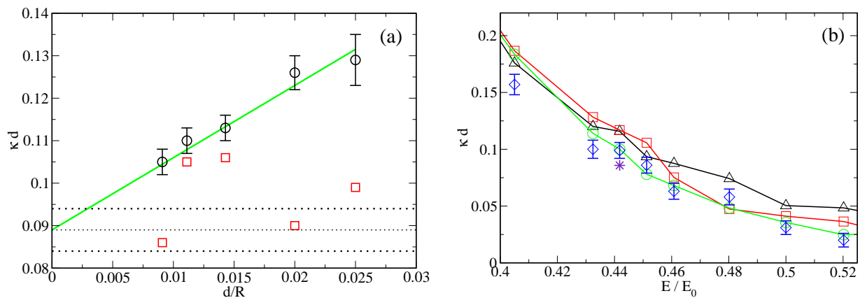
FIG. 2: (Color online) For the 3D system: Comparison of the two methods of calculating the Lyapunov exponent \kappa = 1/\xi . As in Fig.1, the filling factor is p_{\text{occ}} = 1/10 , and the effective scattering length is a_{\text{eff}} = 0.7d . (a) Lyapunov exponent \kappa for a fixed energy of the emitting source, E = \hbar^2 k^2/2m with kd = 0.94 . Red squares: Lyapunov exponent from the first method, see Eq. (10), for several values of d/R ; each point is the result of a fitting on the interval 10d < r < R - 20d . The second method, see Eqs. (13), (14), and (15), leads to a Lyapunov exponent which is the extrapolation at d/R = 0 of the black circles; the green straight solid line is the linear extrapolation, giving \kappa d = 0.089 \pm 0.005 at d/R = 0 ; the three horizontal dotted lines represent the value of \kappa and its confidence interval. The two methods are essentially compatible if one considers the scatter in the data for the first method and the error bars for the second one. (b) For the two methods, Lyapunov exponent \kappa as a function of the energy of the emitting source E = \hbar^2 k^2/2m . The lattice spacing d of the cubic lattice, and the energy E_0 = \hbar^2/(md^2) , are used as units. Note that E_0 = 2E_{\text{rec}}/\pi^2 , where E_{\text{rec}} is the atomic recoil energy after absorption of a lattice photon. Here the filling factor is p_{\text{occ}} = 1/10 , and the effective scattering length is a_{\text{eff}} = 0.7d . The solid lines and the violet star are obtained with the first method [see Eq. (10)]. The three solid lines correspond to sphere radius R = 50d (black line, triangles), R = 60d (red line, squares), R = 70d (green line, circles), and an average over 500 realizations of disorder. The violet star corresponds to a bigger sphere with radius R = 110d , and 100 realizations of disorder. The blue diamond symbols with error bars, are obtained with the second method [see Eqs. (13), (14), and (15)] where the extrapolation has been performed using d/R = 1/50 , d/R = 1/60 , d/R = 1/70 , and 500 realizations of disorder. The second method provides results essentially in agreement with those of the first method. Note the quite small values of the Lyapunov exponents (large localization lengths).
