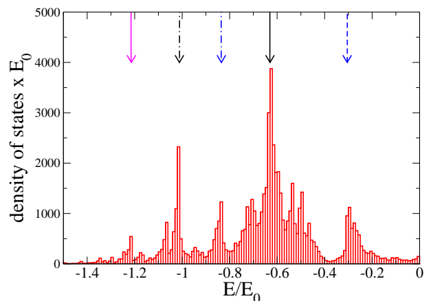
FIG. 16: (Color online) For the 2D system: density of bound states for a given value of the 2D effective scattering length a_{\text{eff}} = d . The histogram is the result of the average over 100 random realizations of the scatterers positions in a disk of radius R = 50d , and a filling factor p_{\text{occ}} = 1/10 . On average, we find 0.85 bound states per scatterer. As done in Fig.15, we also plot the energies of bound states of an A atom with one, two or three B atoms. The vertical lines with arrows indicate the energies of few body bound states AB_n . From left to right are shown the solid magenta line: energy of the tetramer AB_3 Eq.(47) with three B atoms separated by distances r_{13} = r_{23} = d and r_{12} = \sqrt{2}d , dash-dotted black line: energy of a AB_2 trimer Eq.(46) with two B atoms separated by a distance r_{12} = d , dash-dotted blue line: energy of AB_2 with two B atoms separated by a distance r_{12} = \sqrt{2}d , black solid line: energy of a AB dimer Eq.(45), dashed blue line: energy of AB_2 with two B atoms separated by a distance r_{12} = \sqrt{2}d .
