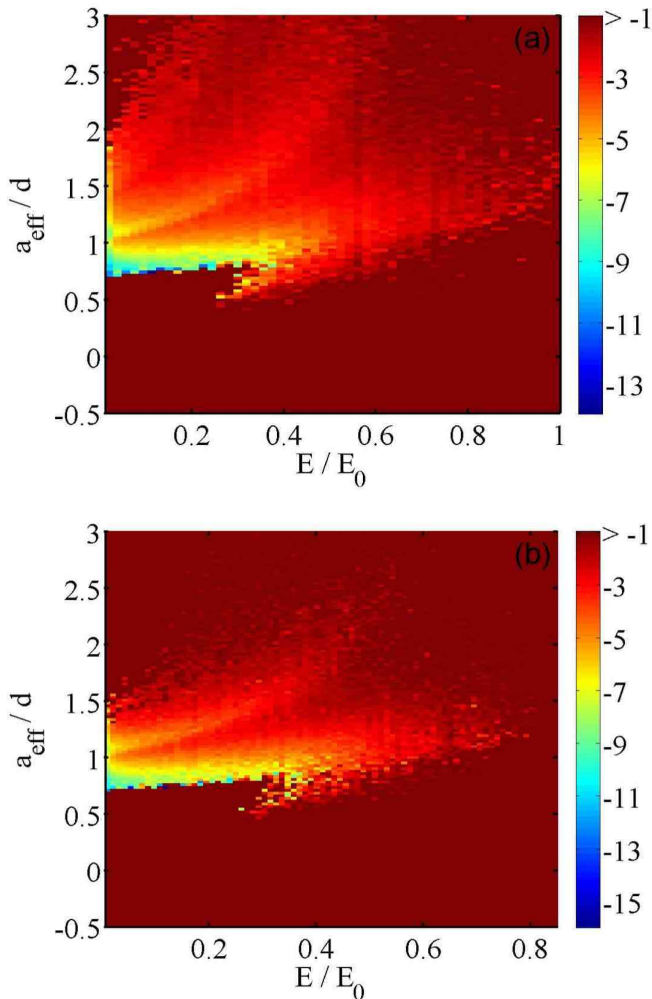
FIG. 11: (Color online) For the 3D system: Width \Gamma of the resonances as a function of the energy E and the effective scattering length a_{\text{eff}} [see Eqs. (24) and (27)]. The physical parameters are the same as in Fig. 7. The plane (E, a_{\text{eff}}) is decomposed in rectangular bins of widths \delta E and \delta a_{\text{eff}} . The color map (see bar on the right) is applied to the quantity \log_{10} \hbar \langle \Gamma \rangle / E_0 where \langle \Gamma \rangle is the mean value of \Gamma for the resonances within a given bin. The resonances are filtered in (a) over the participation volume as in Fig. 7c and in (b) over the r.m.s. size \sigma as in Fig. 7d. In (a) one has \delta E = 0.009 E_0 and \delta a_{\text{eff}} = 0.02d , and in (b) one has \delta E = 0.008 E_0 and \delta a_{\text{eff}} = 0.02d .
