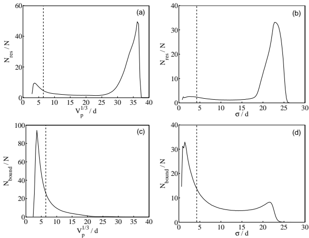
FIG. 9: For the 3D system: For all resonances with E_{\text{res}}/E_0 \in (0, 2) and a_{\text{eff}}/d \in (-3, 3) , and all bound states with E/E_0 \in (-2, 0) and a_{\text{eff}}/d \in (-3, 3) , the figures show an histogram giving the number of resonances (in (a) and (b)) and bound states (in (c) and (d)) per scatterer (the number of scatterers is N = 10^4 ) as a function of: in (a) and (c), the cubic root of the participation volume defined in Eq.(30); in (b) and (d), the r.m.s. size in real space defined in Eq.(31). The bin size is \sim 0.2d for (a) and (c), and \sim 0.26d for (b) and (d). The parameters are the same as in Fig. 7a. The dashed vertical lines are the values V_p^{1/3}/d \simeq 6.5 and \sigma/d \simeq 4.2 [25] used in Fig. 7c and Fig. 7d to select the bound states and resonances that are spatially localized and to filter out the bound states and resonances that are spatially extended.
