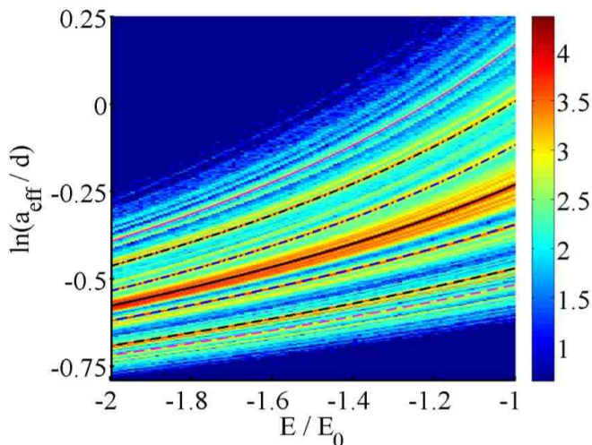
FIG. 15: (Color online) Zoom of figure 14a, in the region of E < 0 (here \delta E = 0.01E_0 , and \delta \ln(a_{\text{eff}}/d) = 0.003 ). On the color map representing the density of states (see caption of Fig.14a), are plotted the energies of bound states of an A atom with one, two or three B atoms, called respectively dimer AB , trimer AB_2 , and tetramer AB_3 . In particular are plotted the energies of a dimer Eq.(45) (black solid line), of a trimer Eq.(46) with two B atoms separated by a distance r_{12} = d (dashed black and dash-dotted black lines), of a trimer with two B atoms separated by a distance r_{12} = \sqrt{2}d (dashed and dash-dotted blue lines), of a tetramer Eq.(47) with three B atoms separated by distances r_{13} = r_{23} = d and r_{12} = \sqrt{2}d (solid and dashed magenta lines). It is worth noting that the predictions for the energies of such isolated bound states correspond to the higher density lines of the color map plot.
