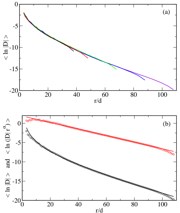
FIG. 1: (Color online) For a source placed at the origin \mathbf{r}_0 = \mathbf{0} , coarse grained histogram giving \langle \ln |D| \rangle as a function of the distance from the source, averaged over 100 realizations of disorder. The lattice for the B atoms is cubic with a lattice constant d , and a filling factor p_{\text{occ}} = 1/10 . The energy of the emitting source is E = \hbar^2 k^2 / 2m with kd = 0.94 . The effective scattering length is a_{\text{eff}} = 0.7d . (a) Coarse grained histogram for 5 different radii R of the sphere containing the scatterers: R/d = 40 (black), R/d = 50 (red), R/d = 70 (green), R/d = 90 (blue), R/d = 110 (violet). (b) For R/d = 110 , coarse grained histogram (black circles) and its fit by the functional form Eq. (10) (black lower solid line), resulting in \kappa d = 0.086 and \alpha = 2.5 ; the same histogram (red circles) and the same fit (red upper solid line) with D_i multiplied by r_i^\alpha . The fit was performed over the interval 10 < r/d < 90 . Note that the largest considered value of R/d = 110 corresponds to a number of scatterers N \simeq 5.6 \times 10^5 .
