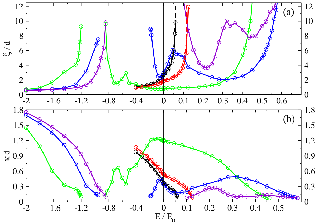
FIG. 4: (Color online) For the 3D system: Localization length \xi [(a)], and Lyapunov exponents \kappa = 1/\xi [(b)], as a function of the energy E of the emitting source for different values of the effective scattering length a_{\text{eff}} : a_{\text{eff}} = 0.1d (black solid line), a_{\text{eff}} = 0.2d (red solid line), a_{\text{eff}} = 0.7d (green solid line), a_{\text{eff}} = d (blue solid line), a_{\text{eff}} = 1.3d (violet solid line). The mean field calculation [see Eq. (18)] is also shown for a_{\text{eff}} = 0.1d (black dashed line), and for a_{\text{eff}} = 0.2d (red dashed line). In (a), for E/E_0 = -1.2 , one has a_{\text{eff}}/d = 1.3, 1, 0.7 from bottom to top, and for E/E_0 = 0.4 , one has a_{\text{eff}}/d = 1, 0.7, 1.3 from bottom to top. The lattice spacing d of the cubic lattice, and the energy E_0 = \hbar^2/(md^2) , are used as units. Results are obtained using the first method [see Eq. (10)], with 500 realizations of the disorder for E > 0 and 100 realizations for E < 0 . The filling factor is p_{\text{occ}} = 1/1 , and the sphere radius is R = 70d , which leads to a mean number of scatterers \langle N \rangle \approx 1.4 \times 10^5 . Comparing the results for E > 0 with 100 and 500 realizations, we estimate that the error on \kappa is \approx 10\% , and even smaller for the lowest values of \xi .
