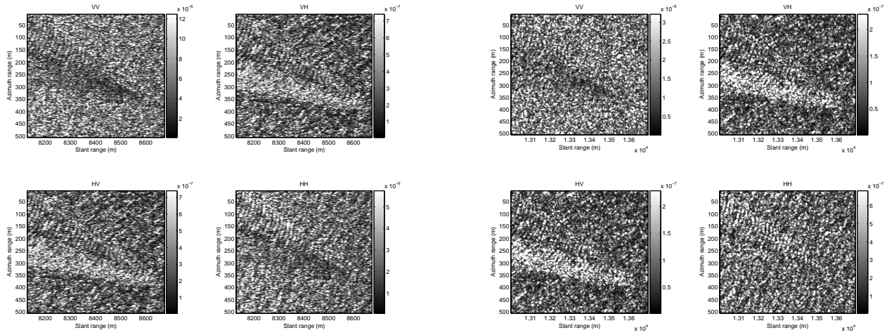
(a) Configuration 1: monostatic SAR, \theta = 45^\circ
