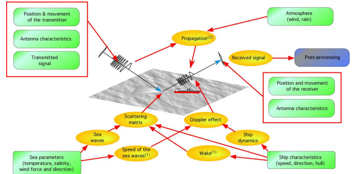
Fig. 1. Simulated configuration. The arrows indicate the dependencies (some of them are omitted for the sake of brevity). (1): partially simulated, non-linear wave interactions not represented, first approximation only for the turbulent wake; (2) not yet simulated. Some relations are omitted for the sake of brevity.
