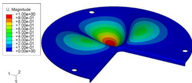
Fig. 14 Deformed shape of the blank corresponding to the third buckling mode obtained during springback
