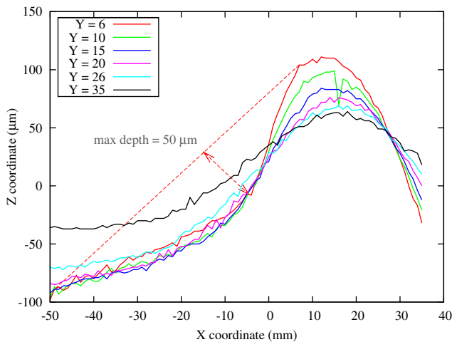
Fig. 6 Profiles along X-axis for different Y values
