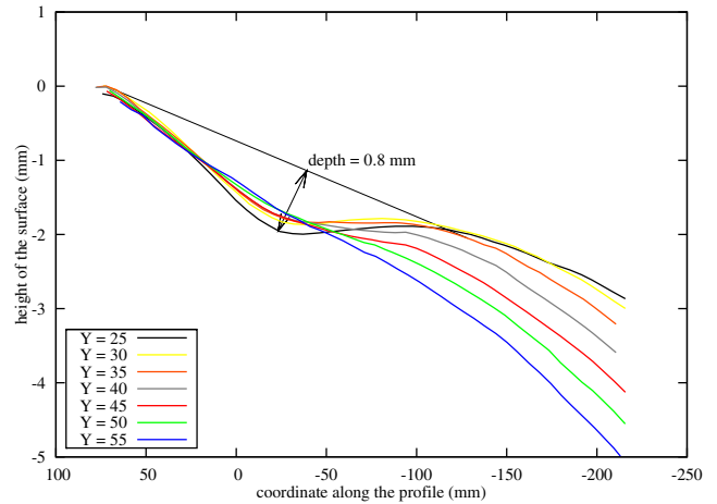
Fig. 8 Profiles after springback for the second refinement at different Y coordinates
