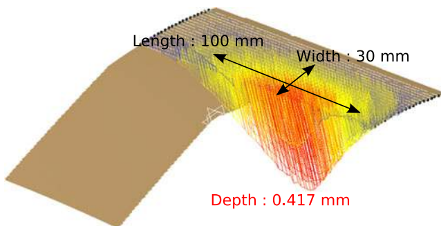
Fig. 2 Estimation of the surface defect size by drawing straight lines on the surface and measuring the gap between the lines and the effective surface
