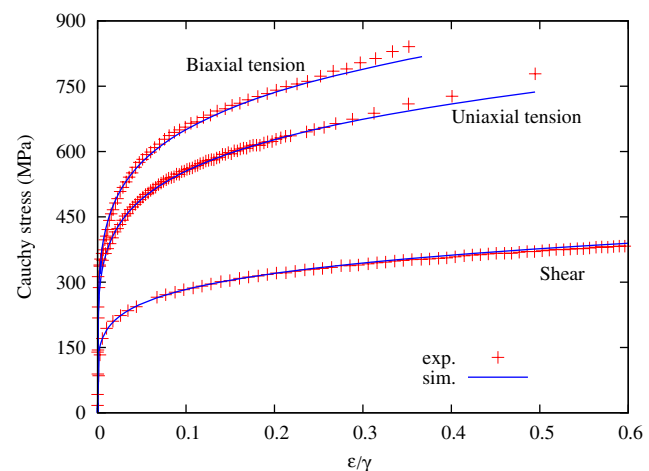
Fig. 7 Comparison of the stress levels between model predictions and experiments for uniaxial tension, simple shear, both in RD, and biaxial tension, for DP500. Similar results are found in the other orientations
