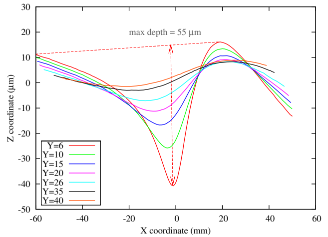
Fig. 11 Profiles along X-axis for different Y values after springback. The simulation is performed with shell elements
