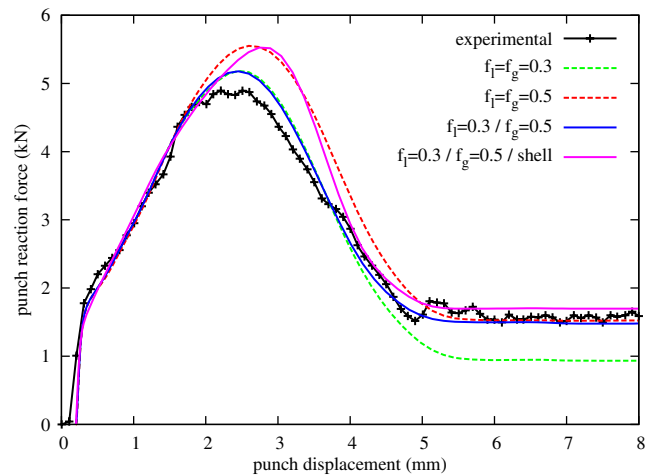
Fig. 9 Comparison of the numerical and experimental punch reaction force with different configurations of numerical friction coefficients for DP500 with a flanged length of 2.5 mm
