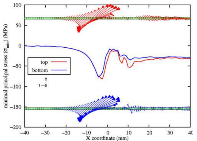
Fig. 12 Distribution of the minimum principal stress (in MPa) in the bottom and top layers of the blank, at Y = 7 mm, for solid elements. The top surface is the one in contact with the blank-holder and the bottom surface with the die. The orientation of the corresponding principal direction is also given
