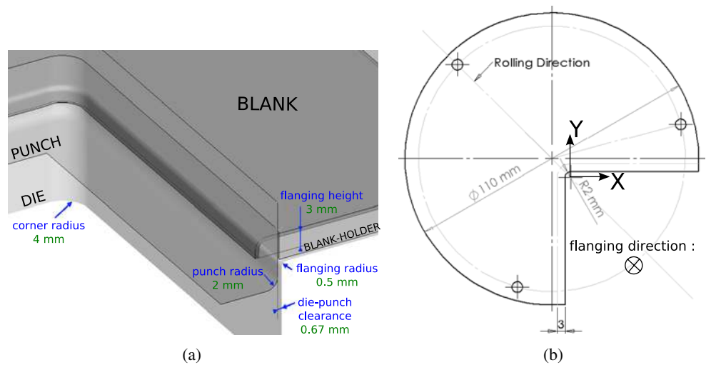
Fig. 5 Geometrical features of the experimental flanging device. a Tools. b Blank
