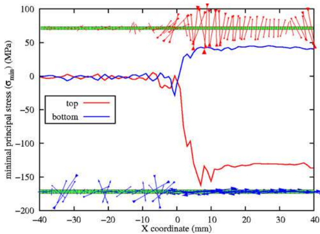
Fig. 13 Distribution of the minimum principal stress (in MPa) at the bottom and top integration points for shell elements ( Y = 7 mm)
