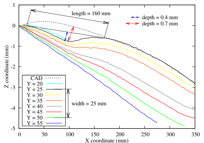
Fig. 4 Profiles of the Atos measurement on the upper corner surface
