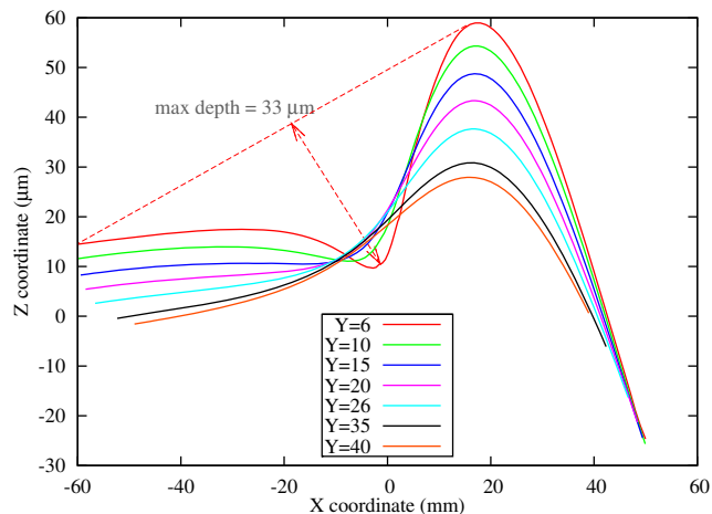
Fig. 10 Profiles along X-axis for different Y values after springback. The simulation is performed with solid elements
