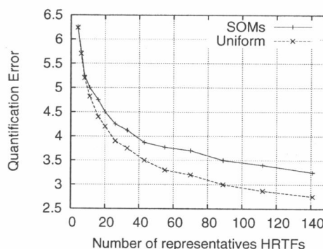
Fig. 6. Average Quantification Error versus the number of representative HRTFs. For all users, the error made with the representatives HRTFs found with SOMs is worse than with the uniformly distributed representatives
