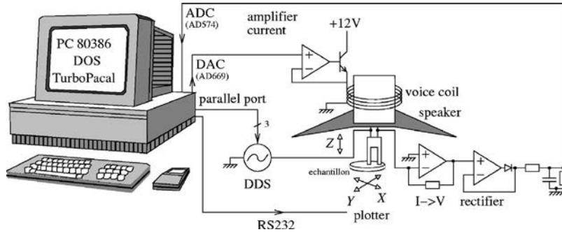
Fig. 5. Experimental setup, including the frequency synthesizer generating the signal for probing the tuning fork and the current to voltage converter, followed by the low-pass filter. Both elements are intended to condition the signal, which is then digitized for computing the feedback current generated by the digital to analog converter. This current, fed to the voice coil, is the quantity later plotted as a function of sample position for mapping the topography of the samples.
