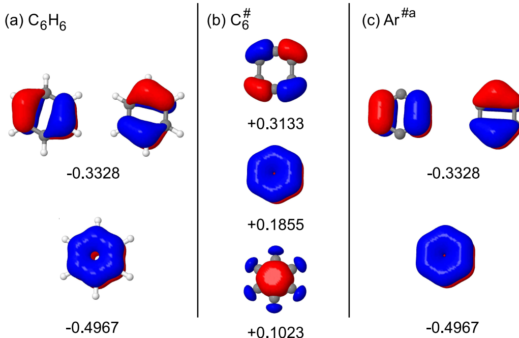
Fig. 1 Design of an \eta^6 - C_6H_6 EGP (a) Reference HF \pi MOs in the 6-31G( d,p ) basis set ; (b) HF MOs obtained in the minimal truncated basis ( i.e. one p GTO / C_6^\# atom, see section 2.1), with carbon ECPs in order to take into account the repulsion of the 1s core, but without the non-local part of \hat{W}_{EGP} ( i.e. without \sum \sum \alpha_{nm} |g_n \gg g_m| ); (c) HF \pi MOs obtained with EGP a . The MO energies are given in hartree.
