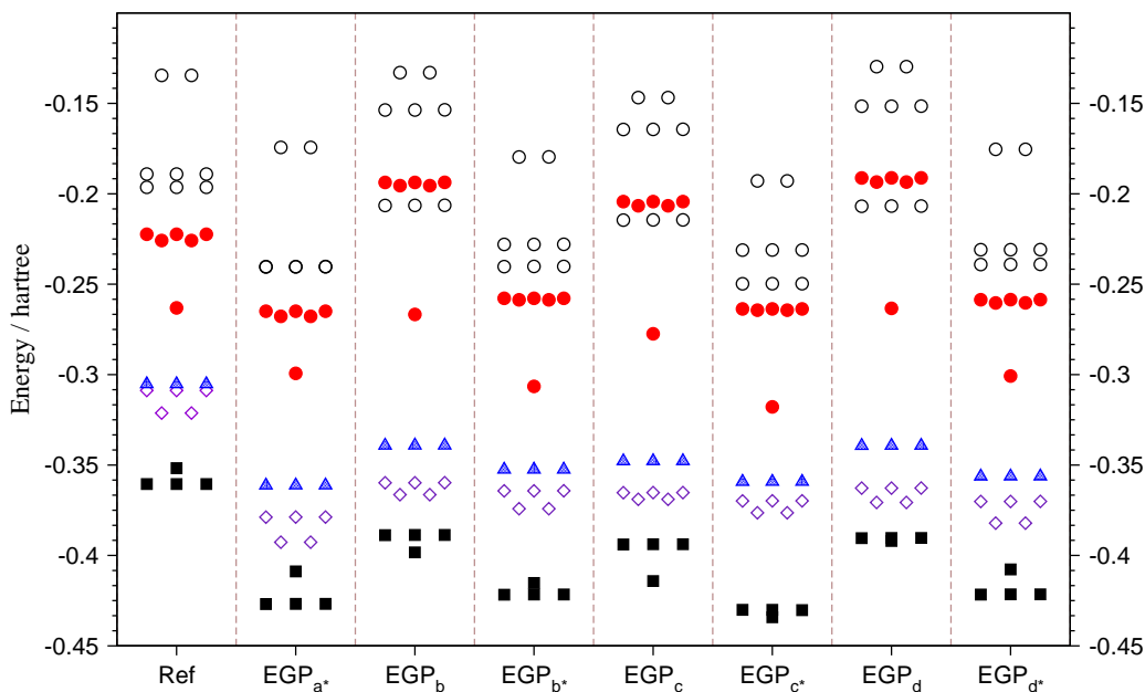
Fig. 4 Energy-level diagrams of the occupied MOs of (\text{H})_4\text{Ru}_4(\text{C}_6\text{H}_6)_4 and (\text{H})_4\text{Ru}_4\text{Ar}^\# close to the Fermi level, calculated for the optimal geometry of (\text{H})_4\text{Ru}_4(\text{C}_6\text{H}_6)_4 . \circ : non-bonding or weakly bonding Ru-Ru MOs ( E and T_2 symmetry); \bullet : skeletal \text{Ru}_4 MOs ( T_1 , E and A_1 symmetry); \blacktriangle : \text{C}_6\text{H}_6 or \text{Ar}^\# MOs; \diamond : \text{C}_6\text{H}_6 -Ru or \text{Ar}^\# -Ru MOs; \blacksquare : Ru-H MOs ( A_1 and T_2 symmetry).
