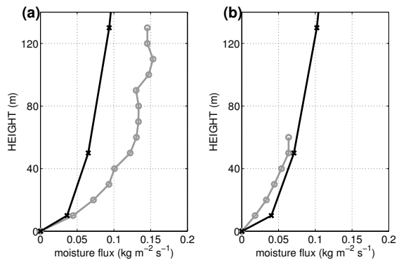
FIG. 8. Mean night time moisture flux ( \mathbf{V}\cdot\mathbf{q}\cdot\rho ) comparisons in \text{kg m}^{-2} \text{s}^{-1} , from the evenings of 11 (a) and 18 (b) August 2005: observations in grey and UM in black.
