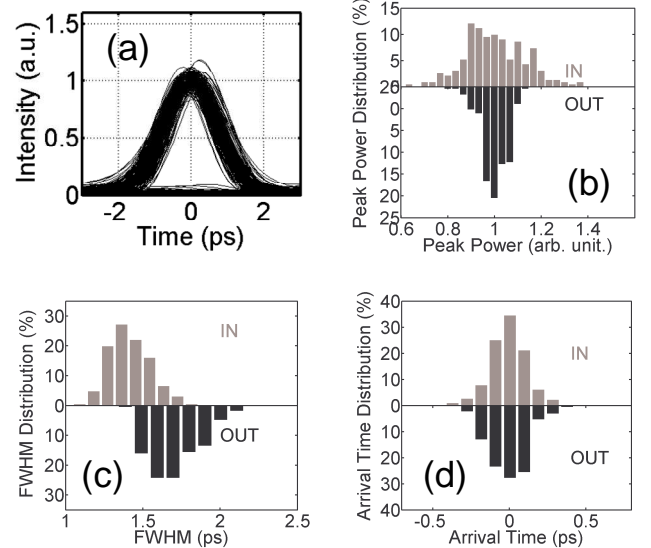
Fig. 10: (a) Output 160-Gbit/s signal for an average power of 14.2 dBm. Statistical distribution of the peak powers (b), temporal width (c) and timing jitter (d) are compared before (grey, top) and after propagation in the power limiter (black, bottom, respectively).
