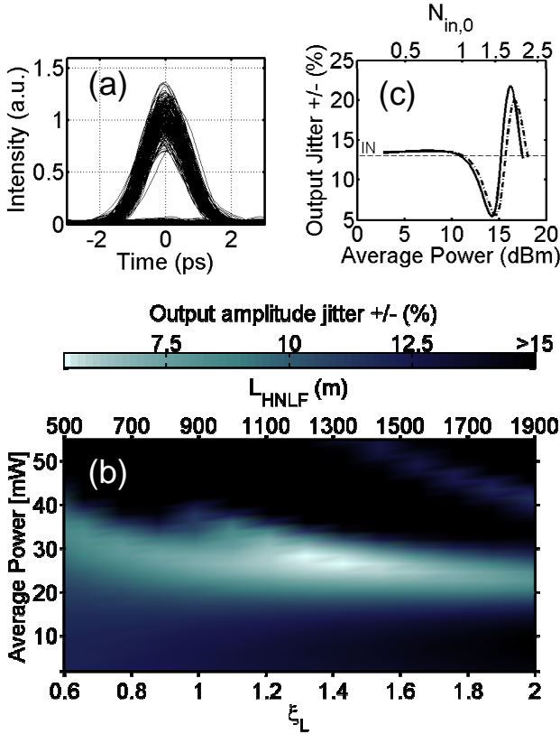
Fig. 9: (a) Input 160-Gbit/s degraded signal (b) Output rms amplitude jitter as a function of \xi_L or L_{HNLF} and average power (c) Output rms amplitude jitter as a function of average power for \xi_L = 1.4 . Dash-dot line, with TOD and fiber losses taken into account in the simulations.
