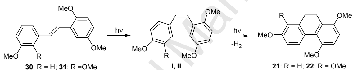
Scheme 3. Photocyclization of stilbenes 30 and 31 to the phenanthrenes 21 and 22 .
