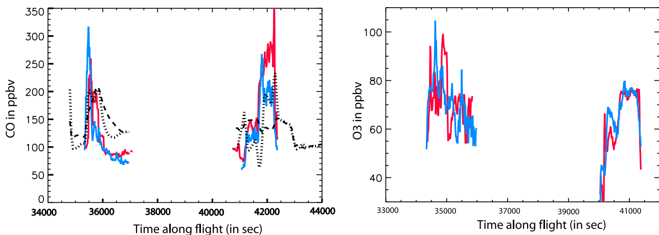
Figure 7. (left) CO and (right) O 3 measured (red lines) and simulated by ZooM-CiTTY (blue lines) on 22 July 2004. MOCAGE CO values with 2 \times 2 and 0.5 \times 0.5 degree resolution are also represented as dashed and dotted black lines, respectively.
