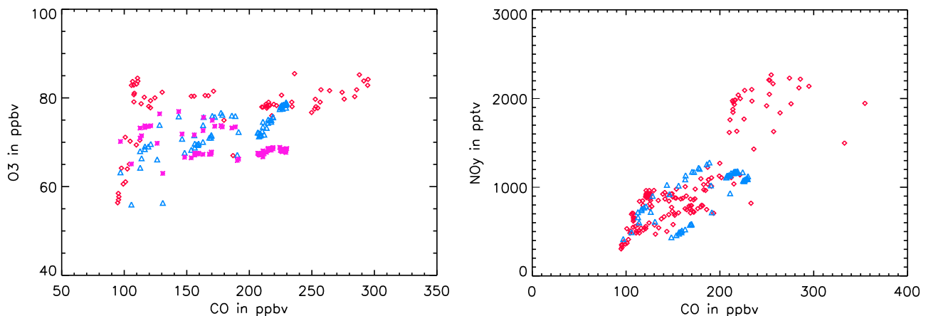
Figure 5. (left) O 3 /CO and (right) NO y /CO correlations measured (red diamonds) and simulated by ZooM-CiTTY (blue triangles) for the plume on 23 July 2004. ZooM-CiTTY O 3 /CO correlations without chemistry are also represented as pink stars in Figure 5 (left).
