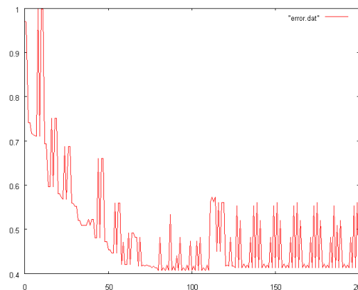
Figure 5. Tabu with 5 elements (best solution \min-e = 0.412 )
