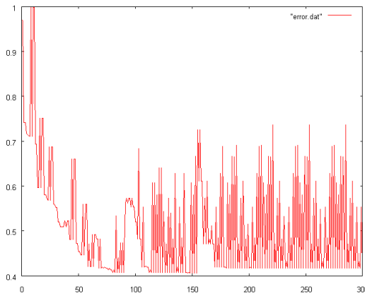
Figure 6. Tabu of size 20 (best solution \min-e = 0.409 )
